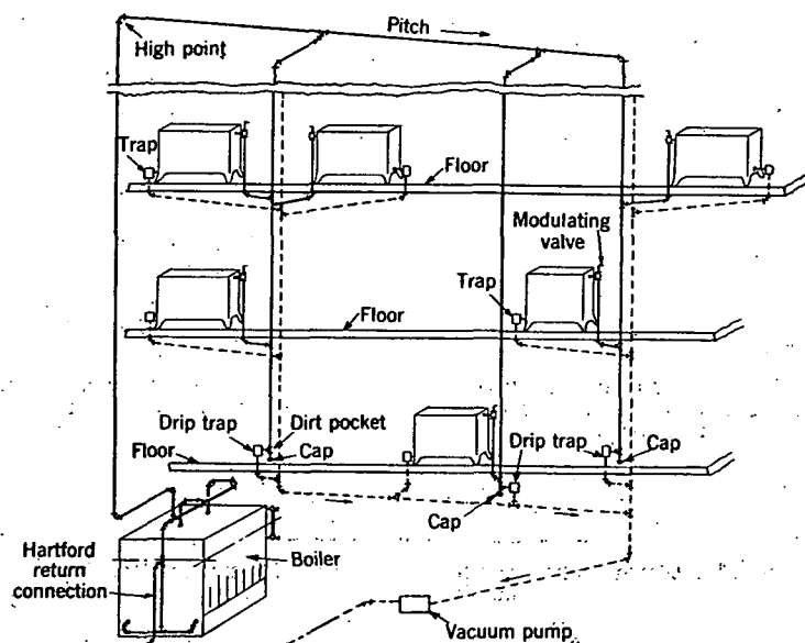
FIG. 18. TYPICAL DOWN-FEED VACUUM SYSTEM
