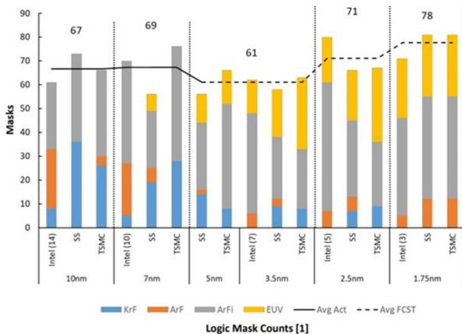
Figure B-6: Layer numbers for advanced logic device nodes by exposure technology.
