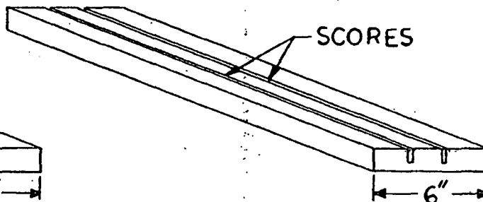
FIGURE 14B - 2 SCORES
