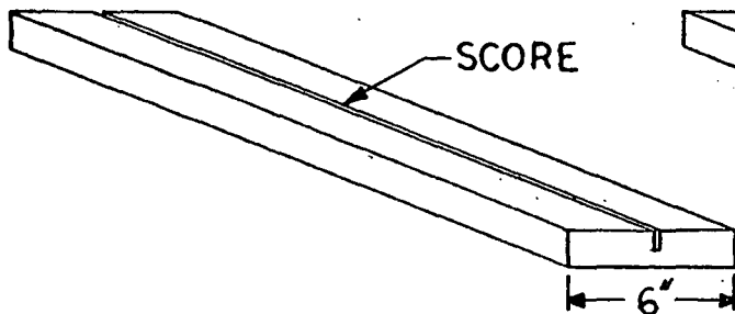
FIGURE 14A - 1 SCORE
