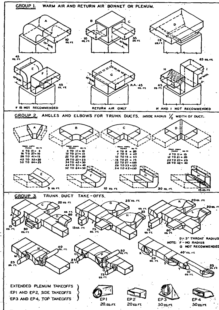
Fig. 7.... Equivalent Length of Fittings and Intakes
