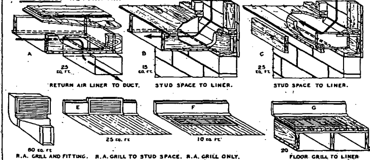
Fig. 7.... Equivalent Length of Fittings and Intakes (Concluded)
