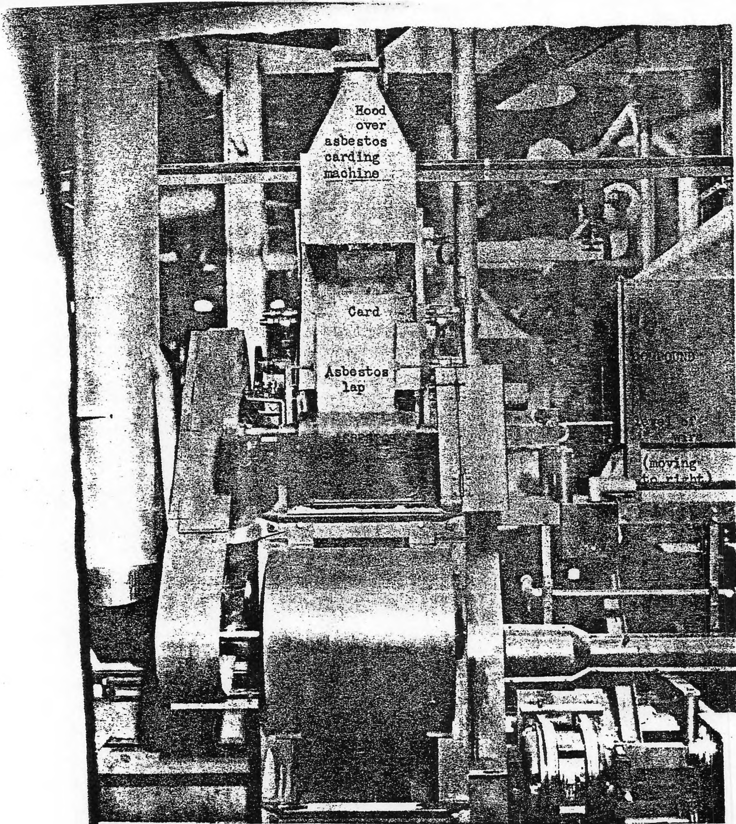
At the York Wire Works (G.E.Co.) is shown a K-Machine. About 50-50 amounts of asbestos and compound are placed upon the wire by this machine. The asbestos is fed and placed upon the wire as a felt. The asbestos dust and waste from this process are removed by the hood shown. This type of wire is used in electric cables, motor leads and fluorescent light fixtures. The steps are (1) asbestos on wire, (2) run through viscous compound, and (3) "polish out" excess compound. The movement of wire through this machine is from left to right.
