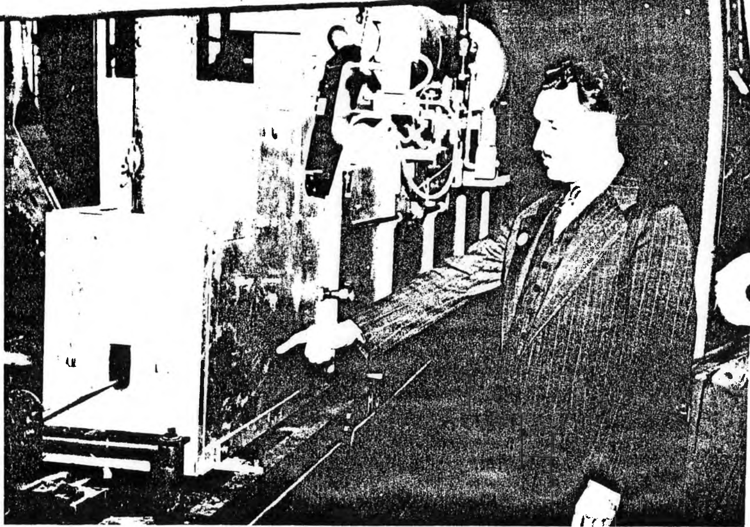
The author of this bulletin is Mr. Fred Kaimer, who is general manager of the York Wire Works division of the General Electric Company's plant at York, Penna. and who is shown standing beside a drying oven, where the solvent alcohol is removed, through the agency of gas fires and ventilation, together with mechanical inclosure. This is an M-Machine and handles the larger diameter wire, usually copper, ranging from 9 gauge (0.114 in.) to 0000 gauge (0.460 in.), American wire standards. The magnet wire is observed as entering the inclosure from the left side through the opening. (In a previous bulletin, Safe Pract. Bulletin #21, Mr. Kaimer has described: Insulation of Wire with Synthetic Wax. Illustrated)
