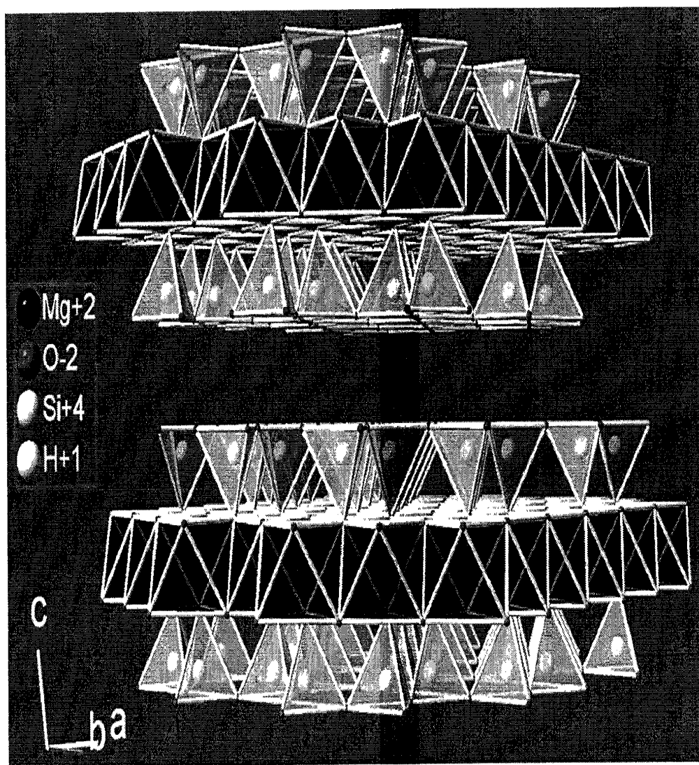
Figure 1.1 Schematic structure of talc
