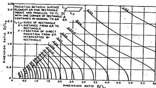
FIG. 4. GEOMETRICAL FACTOR F FOR DIRECT RADIATION BETWEEN AN ELEMENT da AND A PARALLEL RECTANGLE*
