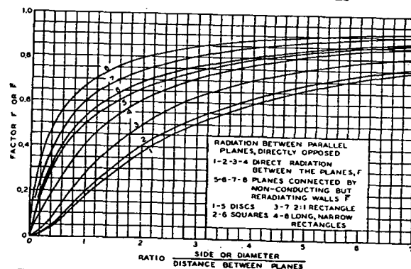
FIG. 6. GEOMETRICAL FACTOR F FOR DIRECT RADIATION BETWEEN OPPOSED PARALLEL RECTANGLE AND DISCS OF EQUAL SIZE*
