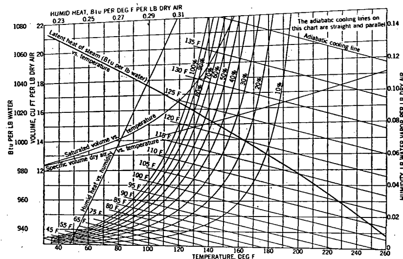
FIG. 6. PSYCHROMETRIC CHART
