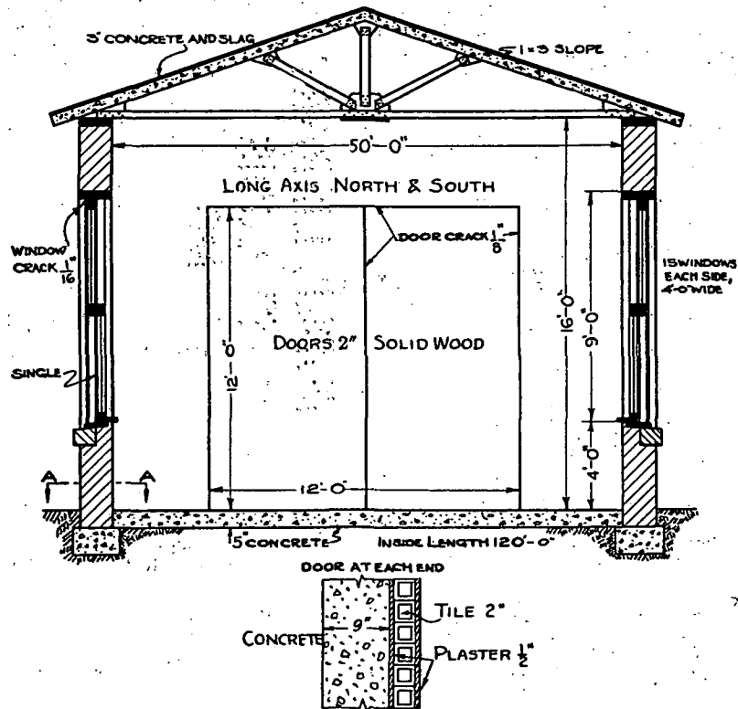
WALL SECTION A-A
