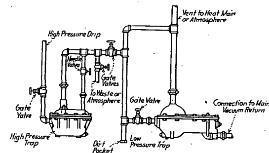
FIG. 3. METHOD OF DISCHARGING HIGH-PRESSURE APPARATUS INTO LOW-PRESSURE HEATING MAINS AND VACUUM RETURN MAINS THROUGH A LOW-PRESSURE TRAP
