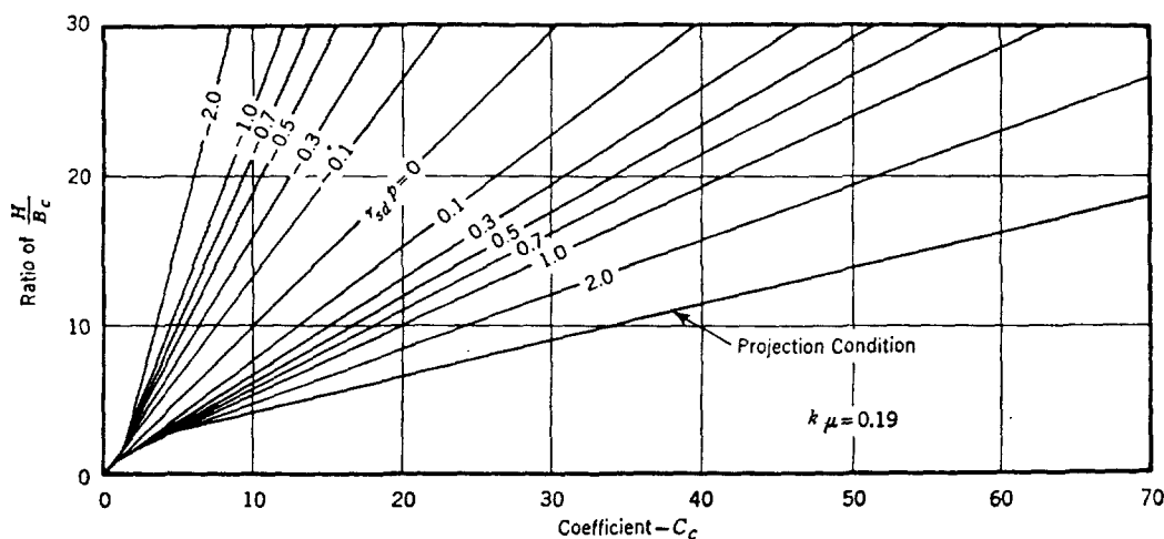
Fig. 3. Graph for Determining Load Coefficient Values
