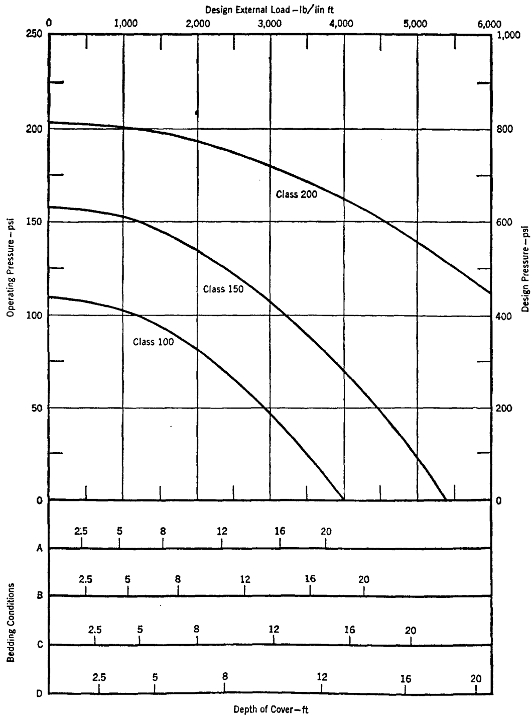
Fig. 8. Selection Curves for 6-in. Asbestos-Cement Pipe
