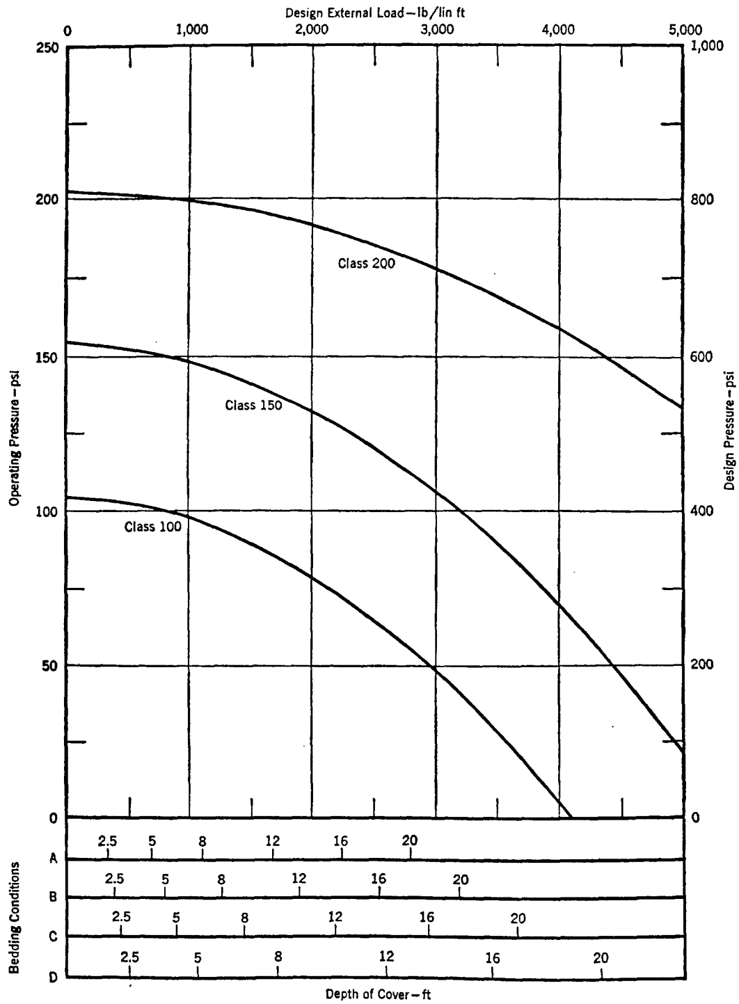
Fig. 7. Selection Curves for 4-in. Asbestos-Cement Pipe
