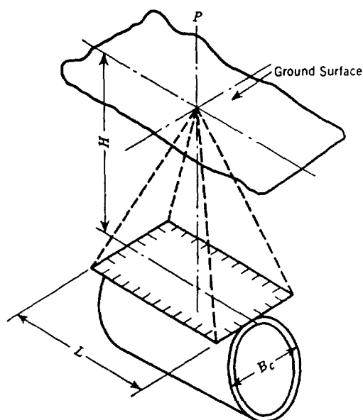
Fig. 5. Concentrated Superimposed Load
