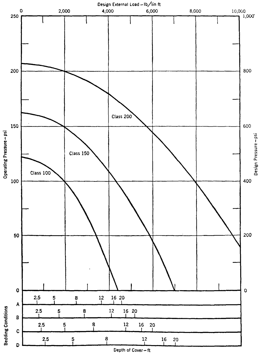
Fig. 10. Selection Curves for 10-in. Asbestos-Cement Pipe
