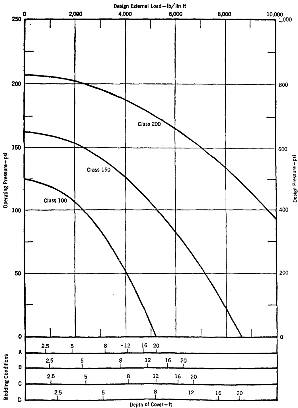
Fig. 12. Selection Curves for 14-in. Asbestos-Cement Pipe
