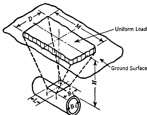
Fig. 6. Distributed Superimposed Load
