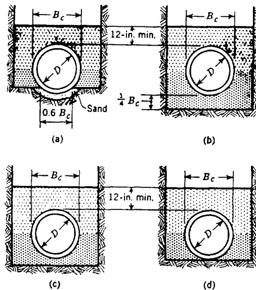
Fig. A2. Bedding Conditions Illustrated
