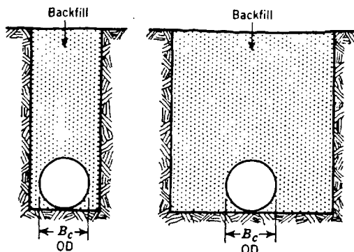
Fig. A1. Earth Load Conditions
