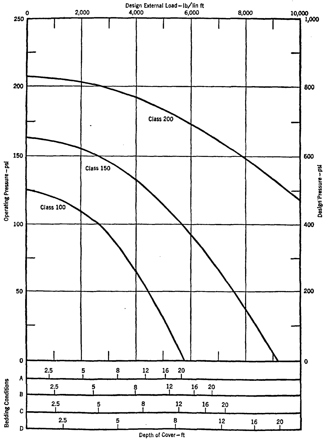
Fig. 13. Selection Curves for 16-in. Asbestos-Cement Pipe
