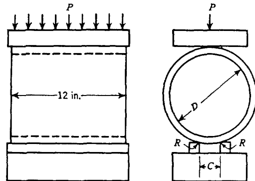
Fig. 2. Crushing Test Assembly
