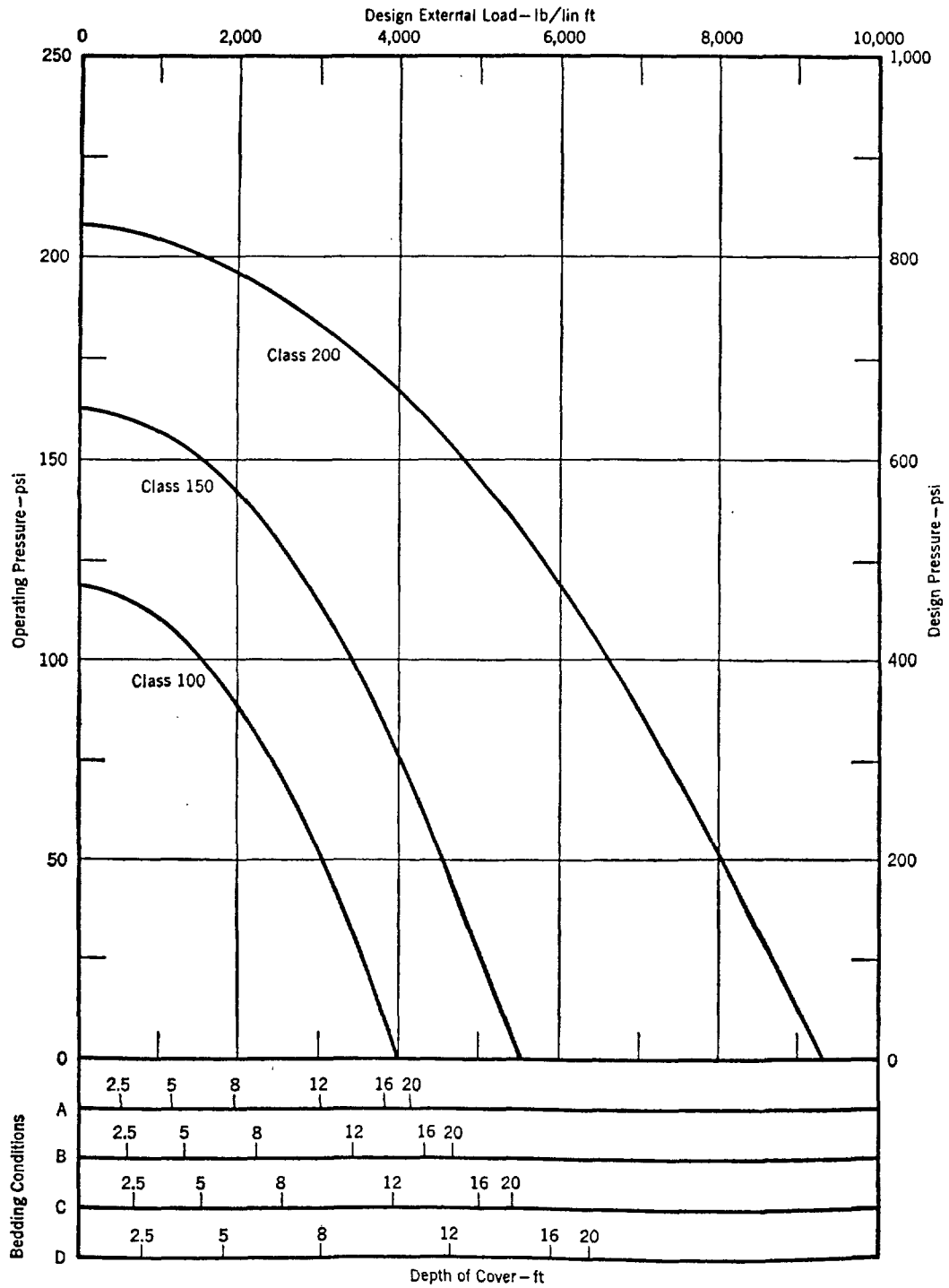
Fig. 9. Selection Curves for 8-in. Asbestos-Cement Pipe
