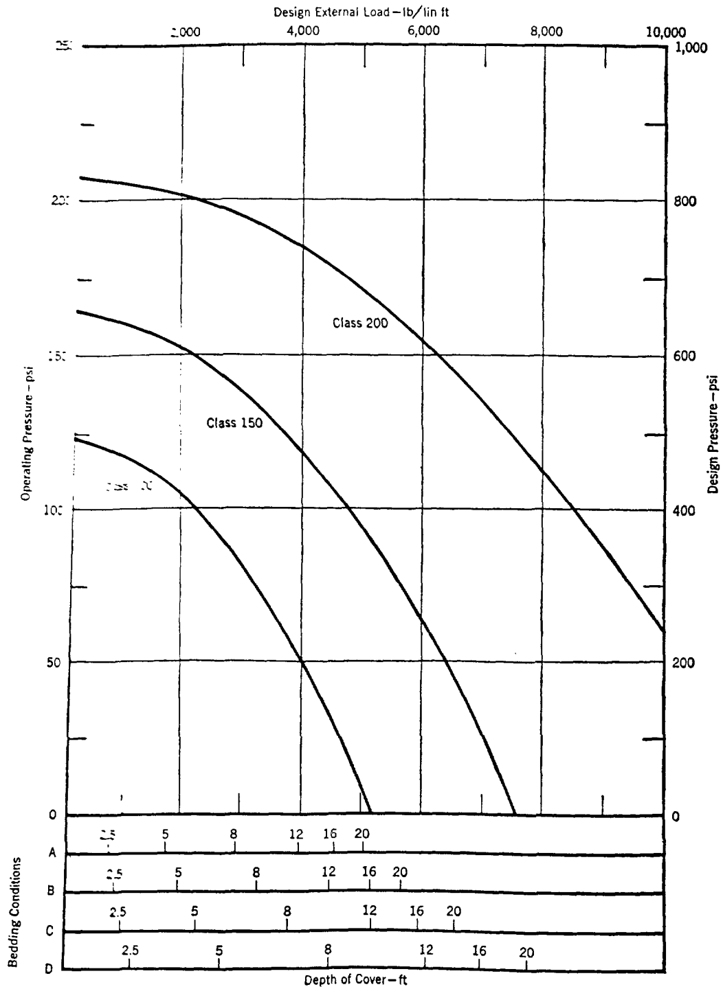
Fig. 11. Selection Curves for 12-in. Asbestos-Cement Pipe
