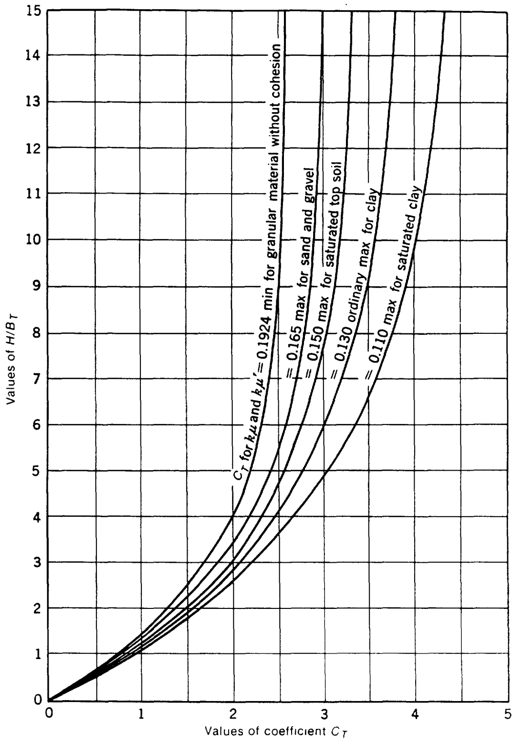
Fig. 12. Values of C_T for Tunnel Conditions
