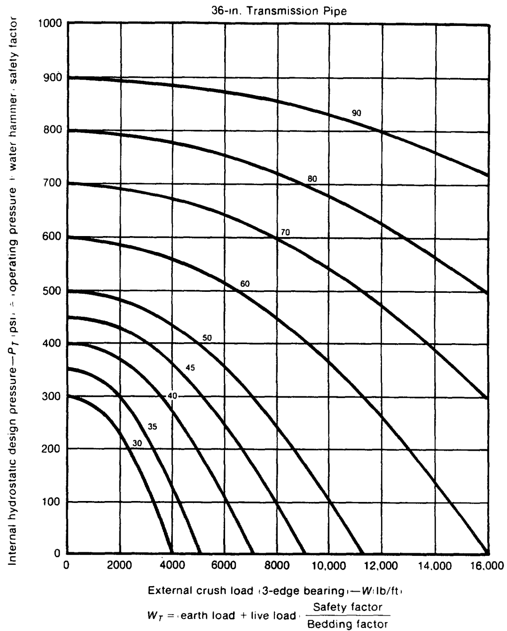
Fig. 14h. 36-in. Transmission Pipe
