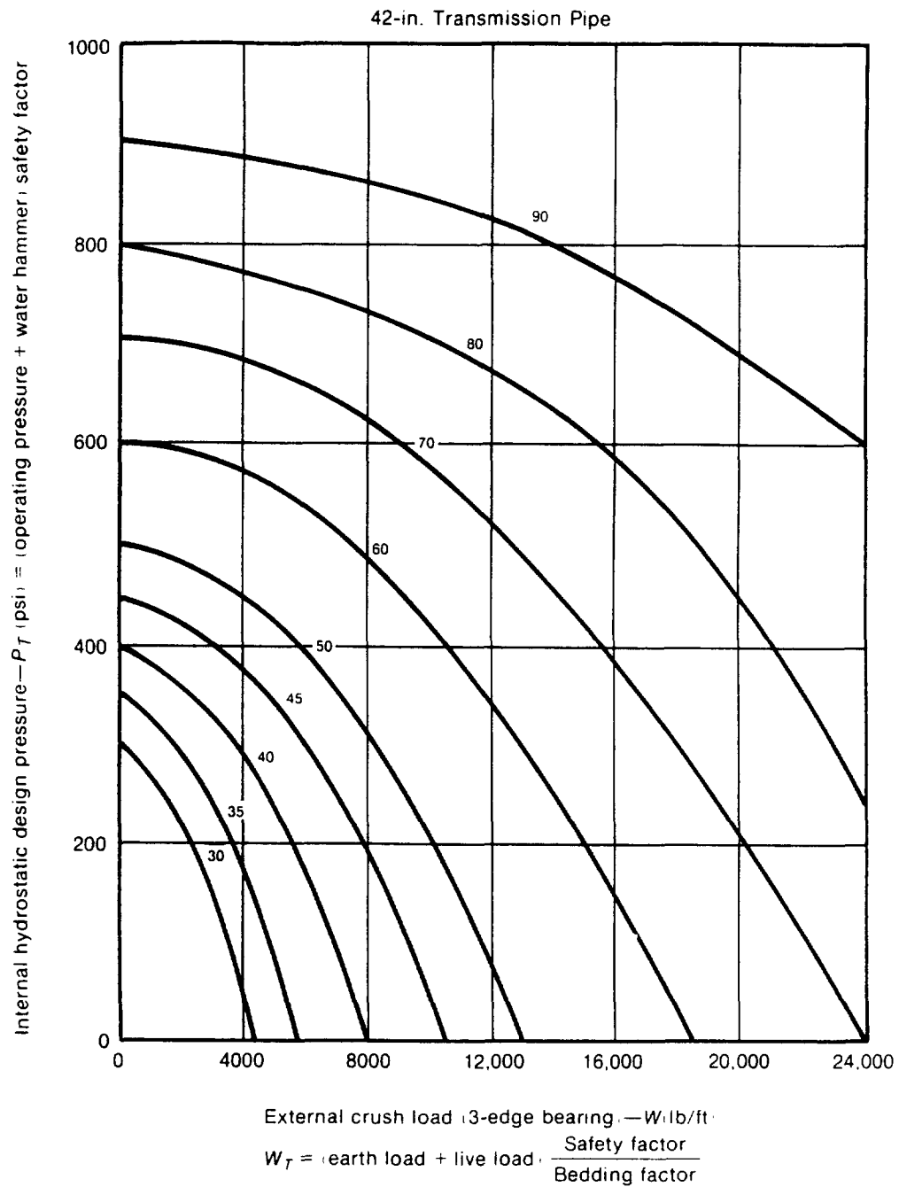
Fig. 14j—42-in. Transmission Pipe
