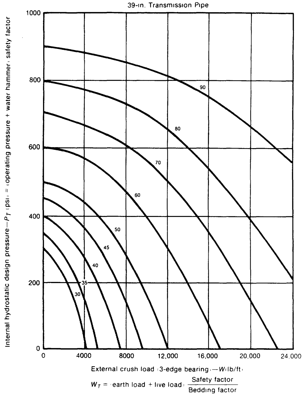
Fig. 14i. 39-in. Transmission Pipe
