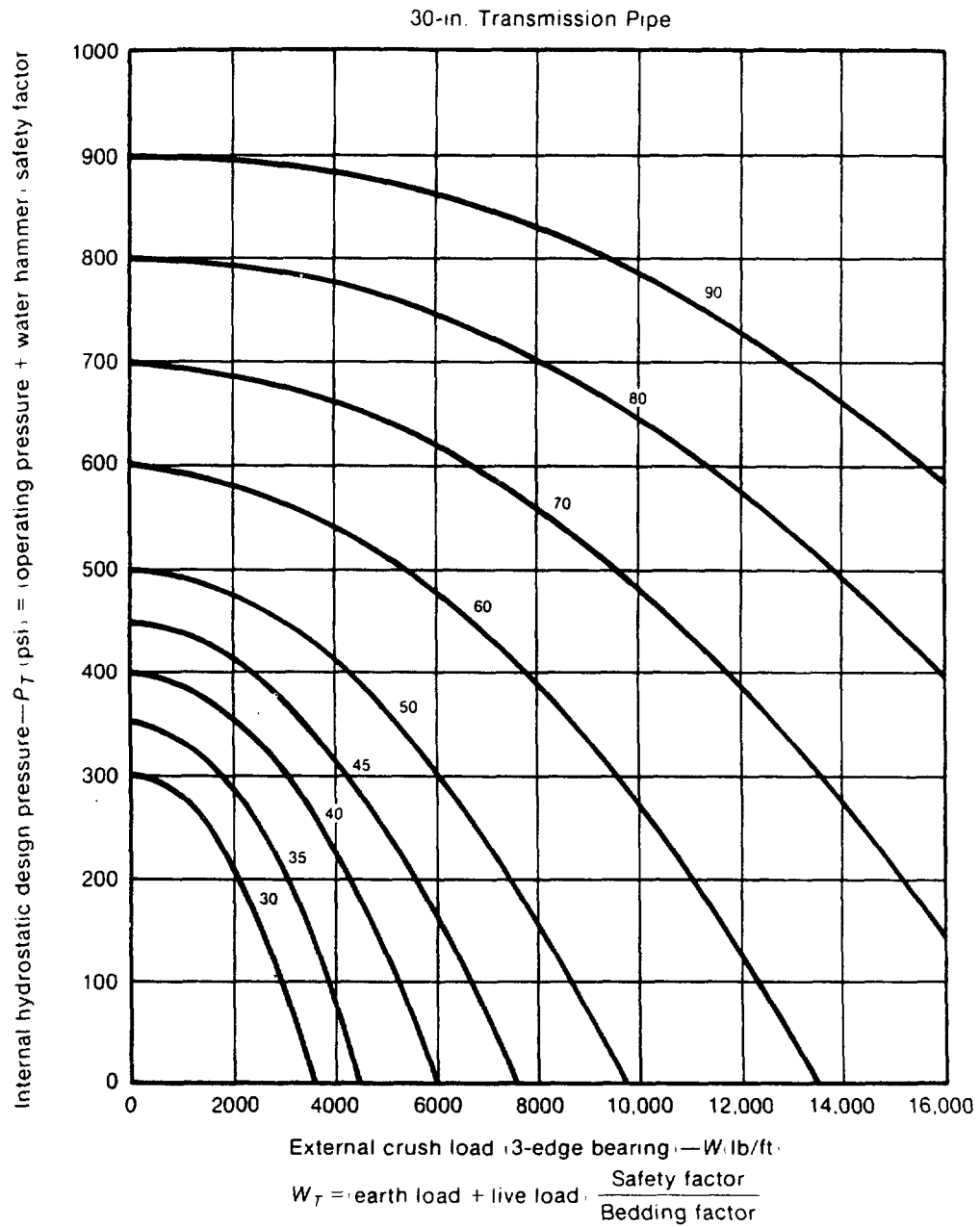
Fig. 14f. 30-in. Transmission Pipe
