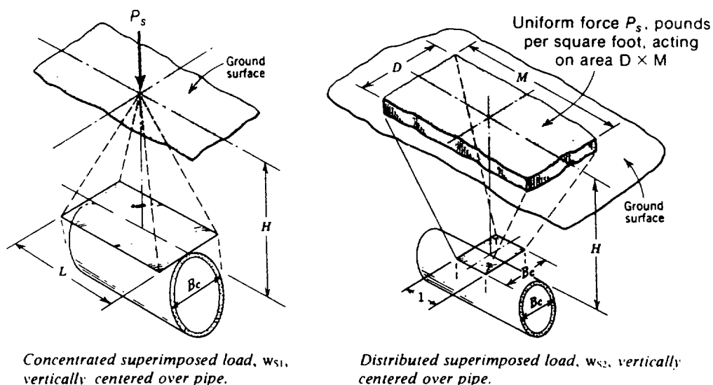
Fig. 13. Superimposed Loads
