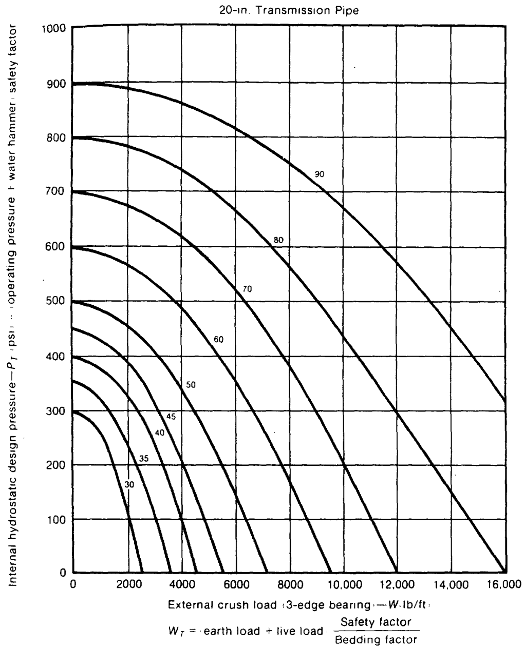
Fig. 14b. 20-in. Transmission Pipe
