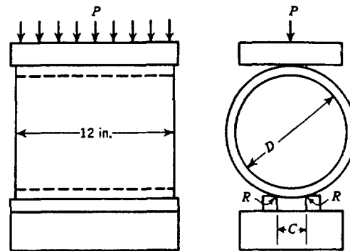
Fig. 3. Crushing Test Assembly
