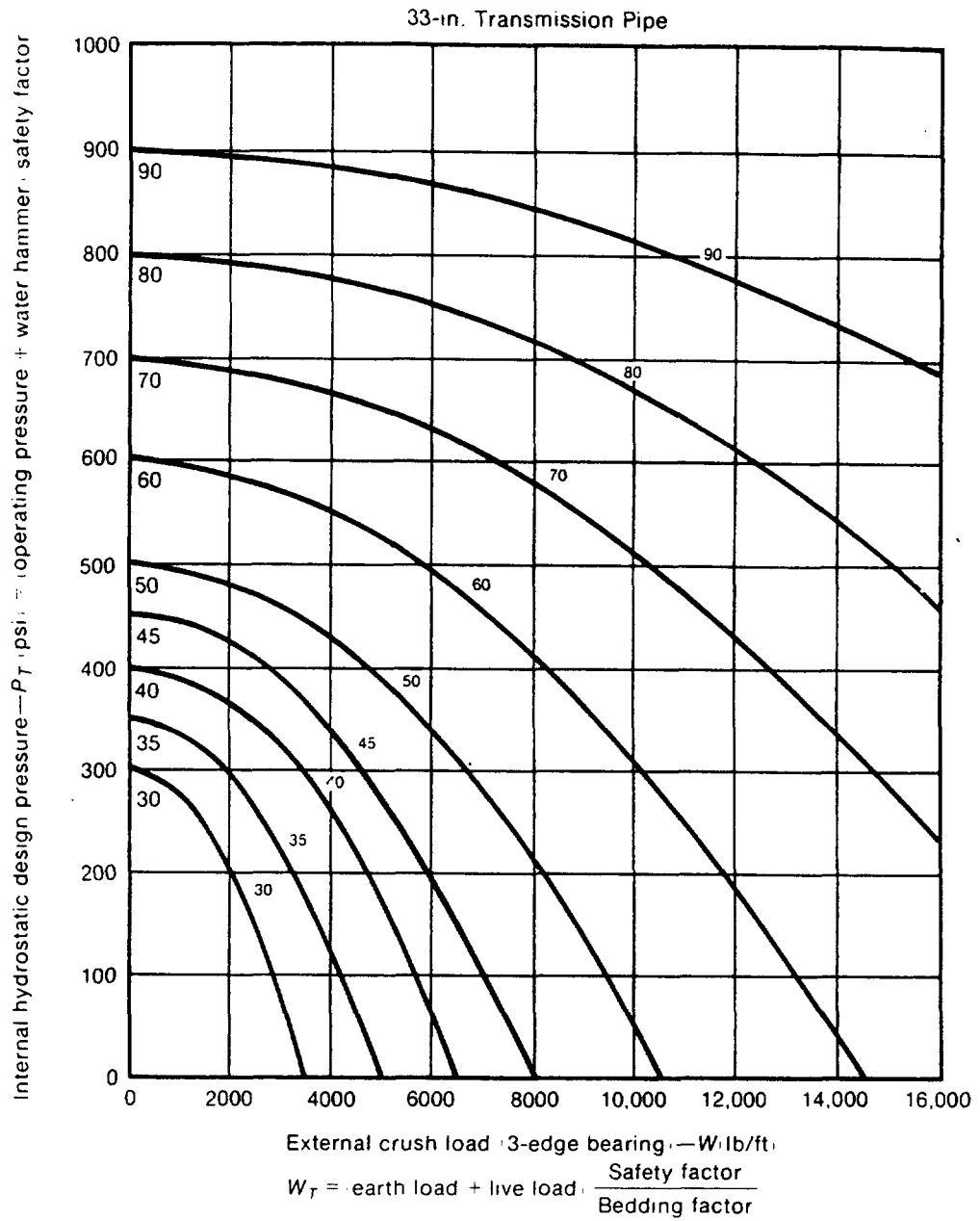
Fig. 14g. 33-in. Transmission Pipe
