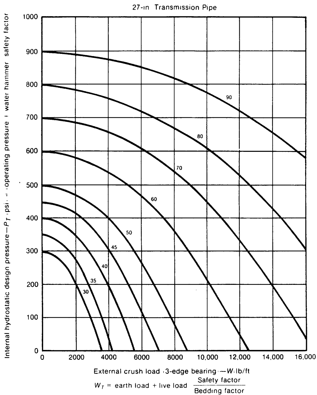
Fig. 14e. 27-in. Transmission Pipe
