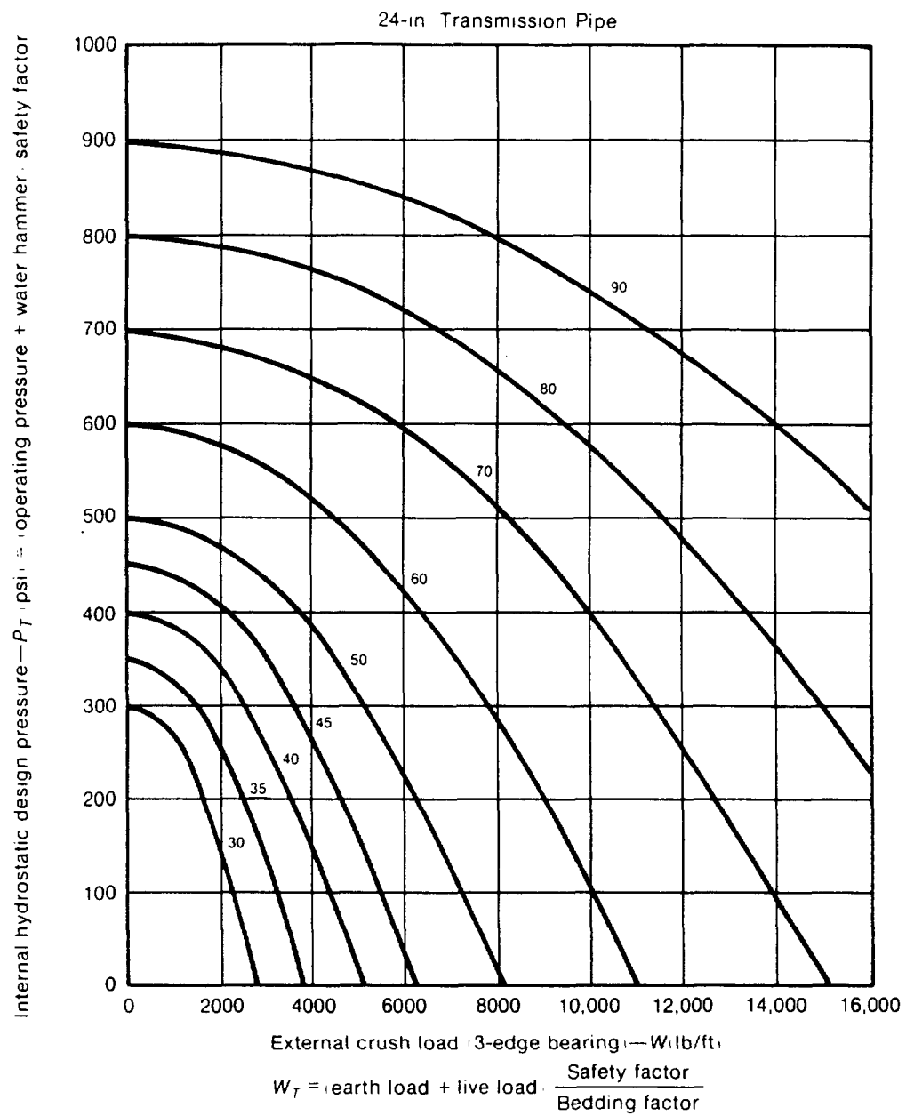
Fig. 14d. 24-in. Transmission Pipe
