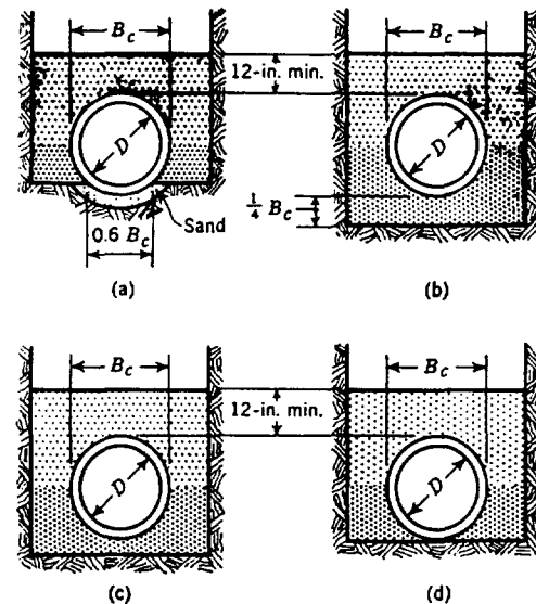
Fig. 1. Bedding Conditions
