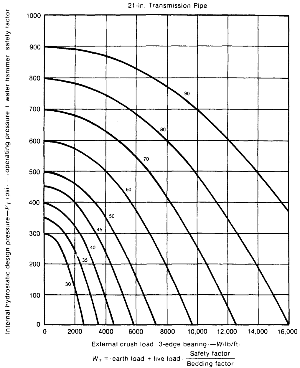
Fig. 14c. 21-in. Transmission Pipe
