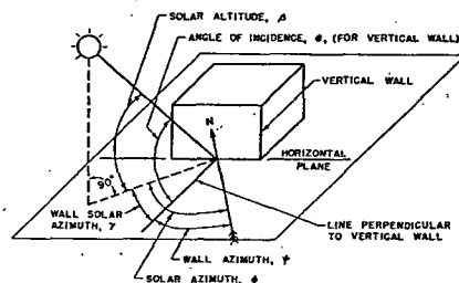
FIG. 1. DEFINITION OF SOLAR ANGLES
