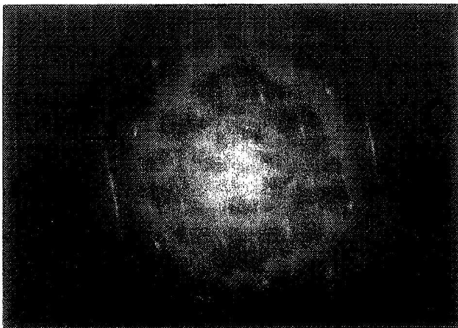
FIG. 1. Electron diffraction pattern of a chrysotile fiber.
