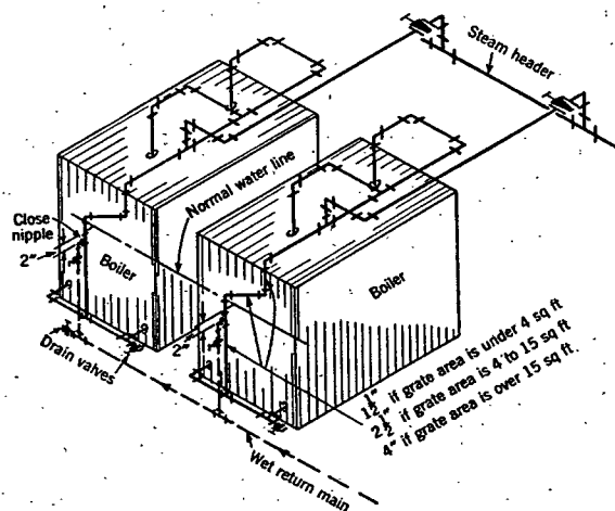
FIG. 3. THE HARTFORD RETURN CONNECTION
