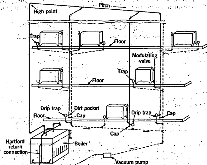
FIG. 15. TYPICAL DOWN-FEED VACUUM PUMP SYSTEM
