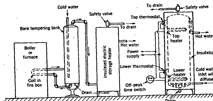
FIG. 7. DOMESTIC HOT WATER HEATER FOR OFF-PEAK SERVICE
