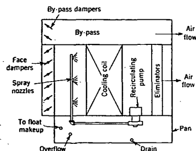
FIG. 11. RECIRCULATING SPRAY SYSTEM FOR CLEANING COILS
