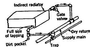
FIG. 11. PIPING CONNECTIONS TO INDIRECT RADIATORS
