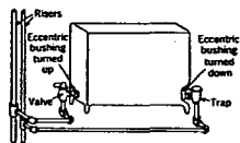
FIG. 6. TYPICAL CONNECTIONS FOR TWO-PIPE SYSTEM
