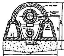
Fig. 6—Single or Double Pipe Lines Using Sectional Pipe Insulation.
