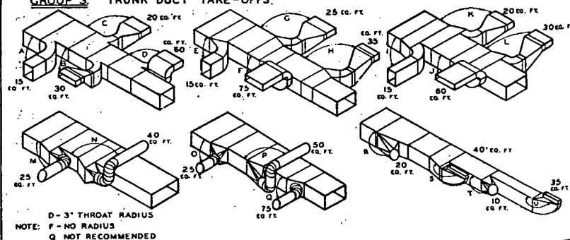
FIG. 7. EQUIVALENT LENGTH OF FITTINGS
