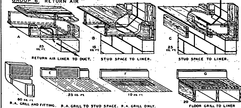
FIG. 7. EQUIVALENT LENGTH OF FITTINGS (Continued)
