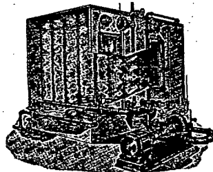
Webster Humidifier Showing circulating pump and spiral spray nozzles by the operation of which air is cleansed, baffles for elimination of free moisture, and automatic devices for the control of temperature and relative humidity
