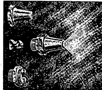
Webster Spiral Spray Nozzle Used in All Atmospheric Installations Also used by meat packers throughout the United States, Canada and South America for spraying brine in meat coolers.
