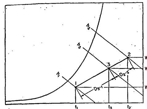
FIG. 11. SOLUTION OF EXAMPLE 5 ON A.S.H.V.E. PSYCHROMETRIC CHART
