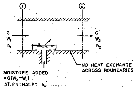
FIG. 12. ILLUSTRATION OF ADDITION OF MOISTURE TO AN ADIABATIC STREAM
