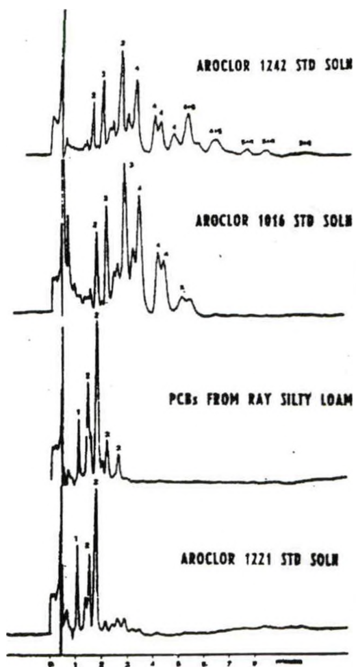
FIGURE 2. PCB ELECTRON CAPTURE GAS CHROMATOGRAMS
