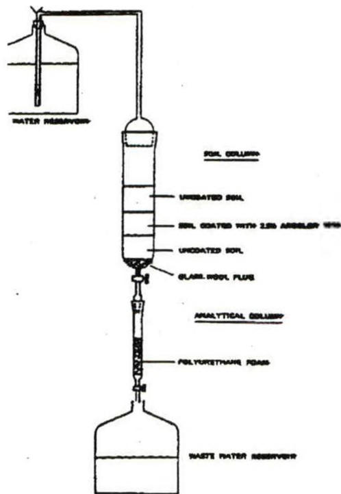
FIGURE 1. SOIL PERCOLATION SETUP
