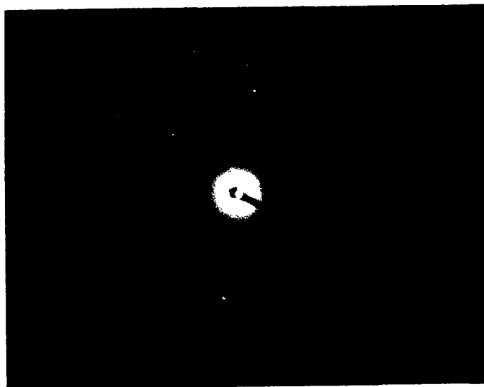
Diffraction Patterns
