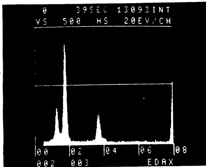
X-Ray Spectrum
