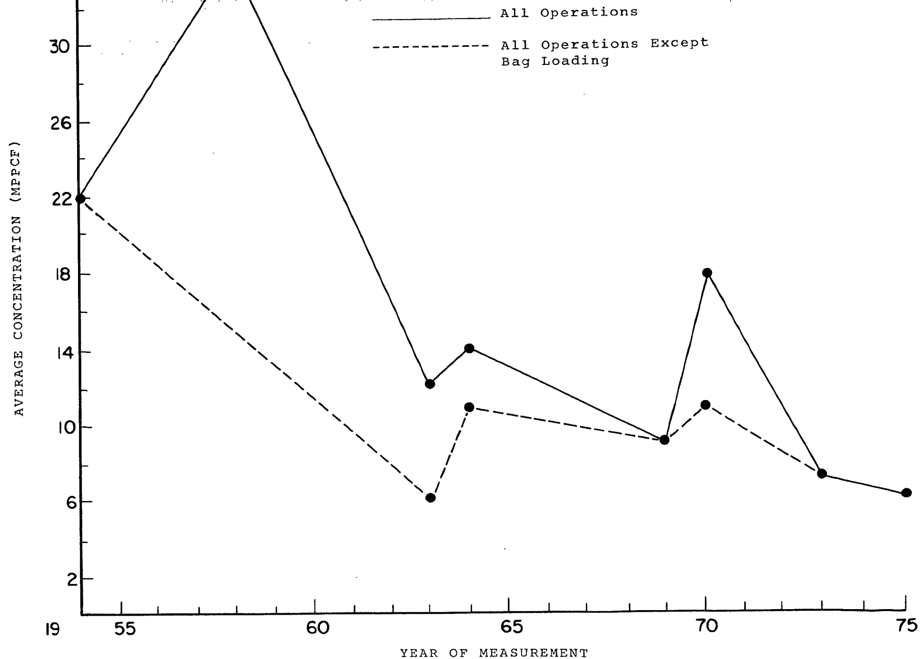
Figure 7. Mean Yearly Impinger Dust Concentrations for Mill Operations
