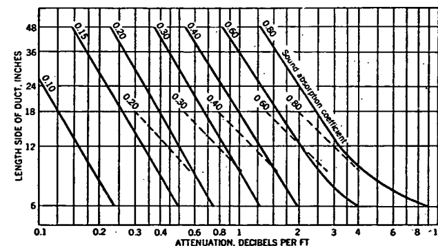
FIG. 5. SOUND ATTENUATION FOR VARIOUS ABSORBING DUCT LINERS
