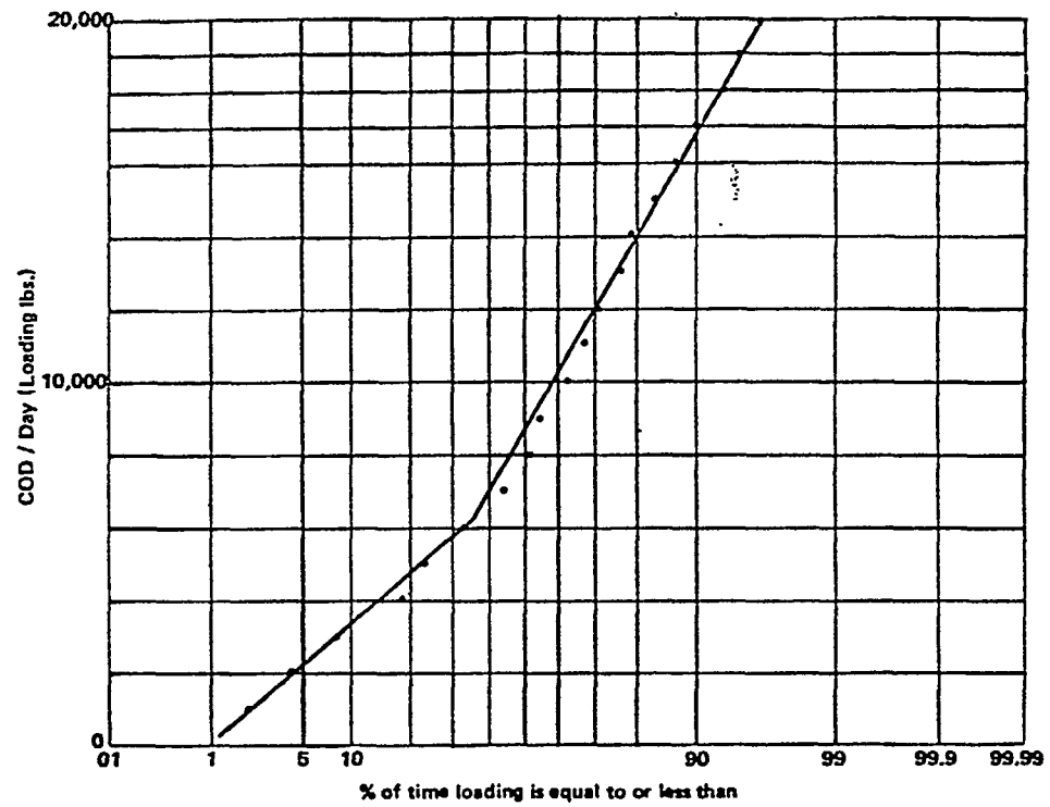
Figure 8-7c. PROBABILITY OF OCCURRENCE OF TOMATO WASTE LOADING
