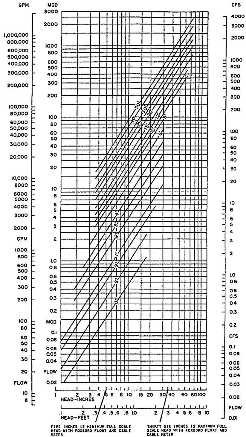
Figure 7-19. FLOW CURVES FOR PARSHALL FLUMES
