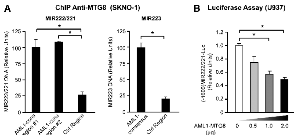
Figure 4. MIR-222/221 transcriptional repression by the CBFL fusion protein AML1-MTG8. (A) ChIP with anti-MTG8 showing that endogenous AML1-MTG8 is bound significantly more to the AML1-consensus sequence-containing regions present in the MIR-222/221 and MIR-223 promoter relative to a control region in the t(8;21)-positive SKNO-1 cell line. (B) Reporter assay showing that luciferase expression driven by the MIR-222/221 promoter (from –1600 to +1) is significantly repressed by expression of exogenous AML1-MTG8 in U937 cells.
