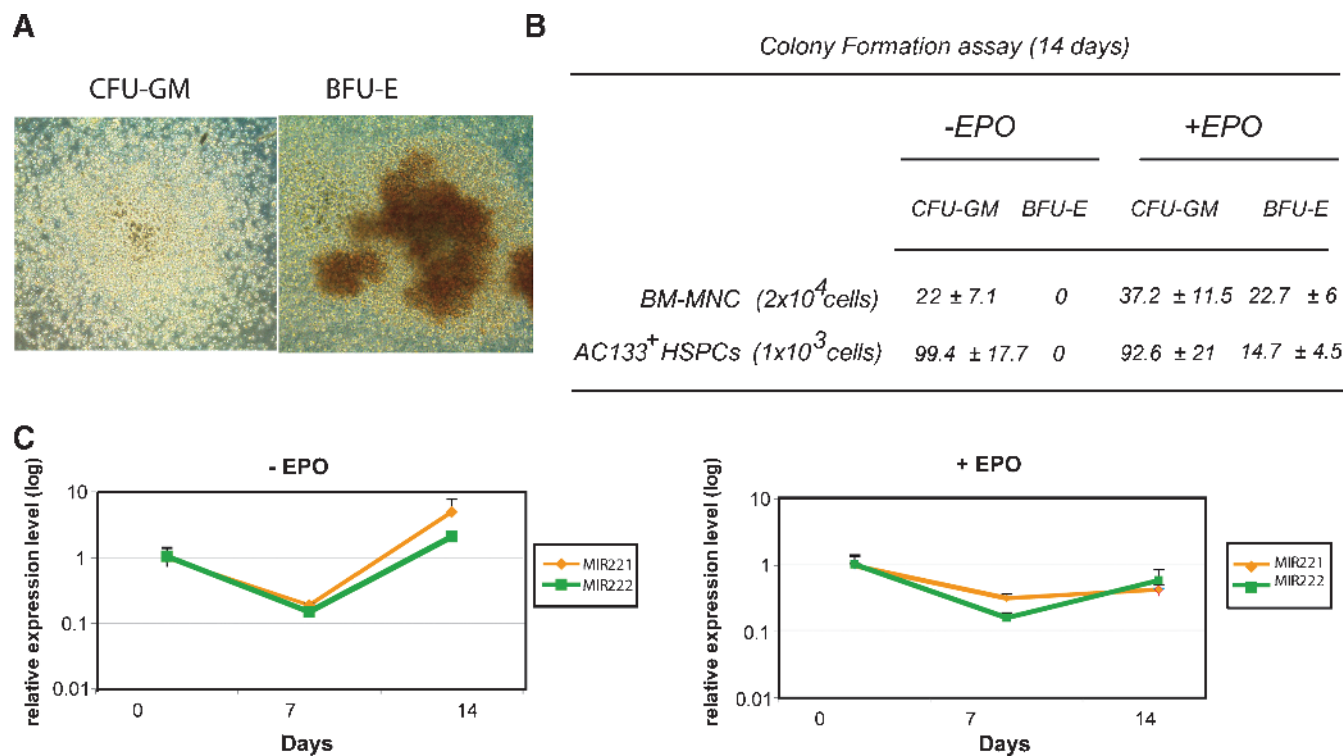
Figure 3. Up-regulation of MIR-222/221 during AC133 + HSPCs in vitro granulocyte/macrophage differentiation. (A) Representative CFU-GM (left) and BFU-E (right) colonies formed by AC133 + HSPCs isolated from the BM-MNCs of the healthy donor, after 14 days in a colony formation assay in the absence or presence of EPO, respectively. (B) Colony quantitative/qualitative analysis shows that AC133 + cells form significantly more CFU-GM colonies than BM-MNC after 14 days of culture in the presence or absence of EPO. (C) CFU-GM induction of AC133 + cells followed by real-time stem-loop RT-PCR shows up-regulation of MIR-222/221 after 14 days (left), whereas no significant differences in MIR-222/221 expression could be detected when BFU-E and CFU-GM were concomitantly induced by culturing AC133 + cells for up to 14 days in the presence of EPO (right).
