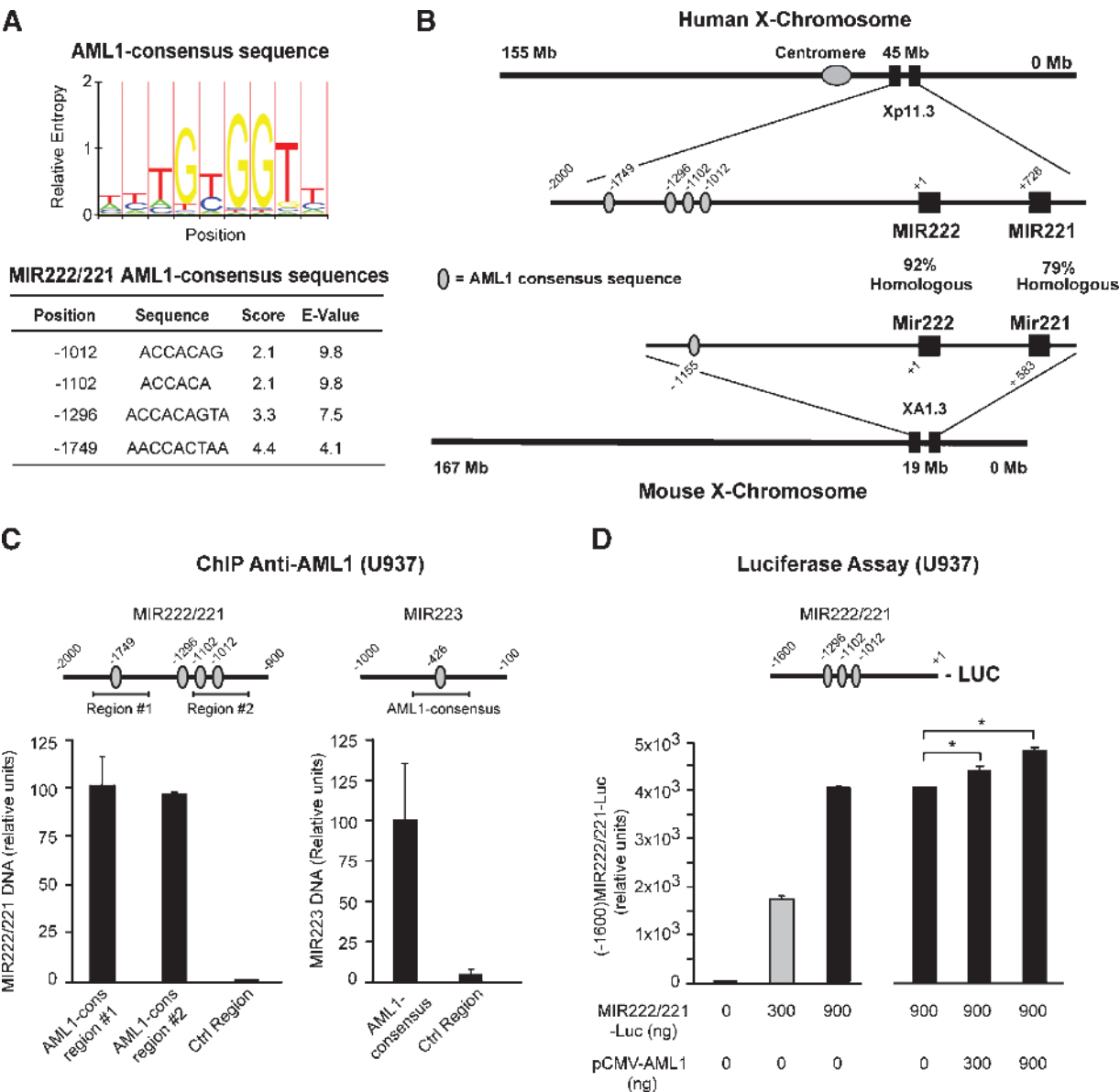
Figure 1. AML1 is implicated in the transcriptional control of MIR-222/221. (A) “Logo” representation of the most probable nucleotide combinations of the AML1-consensus sequence (top). Four AML1-consensus sequences could be identified on the minus strand (the transcribed strand) of the 2-kb region upstream of the MIR-222/221 transcription start site (bottom). (B) Scheme showing the relative position of the putative AML1-binding sites identified by in silico analysis of the human and mouse MIR-222/221 cluster. (C) ChIP with anti-AML1 showing that endogenous AML1 is bound significantly more to the AML1-consensus sequence-containing regions present in the MIR-222/221 and MIR-223 promoter relative to a control region in U937 cells. (D) Reporter assay showing that luciferase expression driven by the MIR-222/221 promoter (from –1600 to +1, see top panel) was induced in U937 cells (left) and was significantly enhanced by the expression of exogenous AML1 (right).
