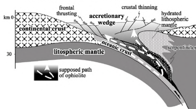
Fig. 2. Schematic scenarios of tectonic settings for ophiolites. (a) Mantle exhumation and ophiolite formation during two main crustal mechanisms: lithospheric detachment (e.g. McKenzie and Bickle, 1988, redrawn and modified) and coaxial stretching at the mid-oceanic ridge (e.g. Whitmarsh et al., 2001, redrawn and modified). (b) Subduction-exhumation setting illustrating possible tectono-metamorphic events experienced by ophiolites (after Agard et al., 2009, redrawn and modified). (c) Ophiolite obduction along a regional-scale metamorphic sole thrust (after Searle et al., 2003, redrawn and modified).
