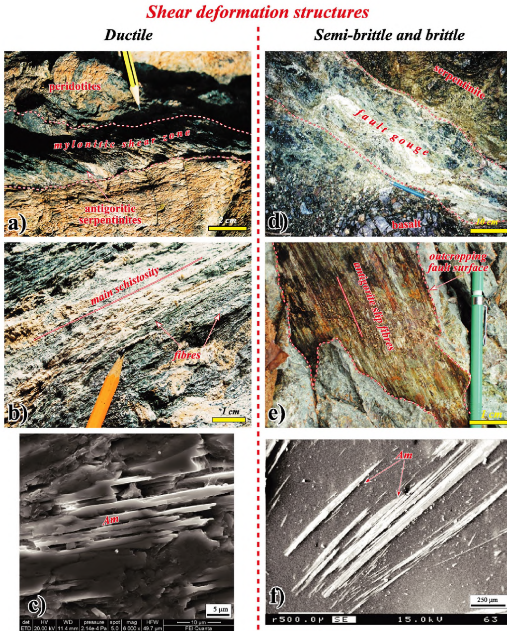
Fig. 5. Examples of ductile and brittle shearing in ophiolites. (a) Meso-scale ductile mylonitic shear zone with development of serpentinites in massive herzolites; (b) meso-scale pervasive schistosity in serpentinites accomplished by occurrence of free asbestiform minerals (probably tremolite); (c) SEM image of strongly aligned amphibole in foliated microfabric; (d) decimetric-width fault gouges in serpentinites with fine-grained antigorite (the white horizons); (e) antigorite slip fibres developed on fault surface in metagabbros; (f) BSE images of fibrous amphiboles showing fracturing in parallel thinner fibres. Mineral abbreviation: Am: amphibole.
