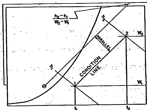
FIG. 16. SOLUTION OF EXAMPLE 8 ON A.S.H.V.E. PSYCHROMETRIC CHART
