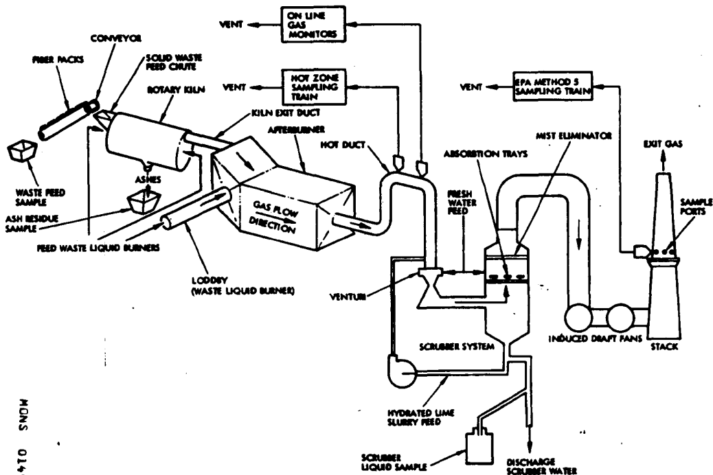
Figure 5-7. Schematic of Rollins Environmental Services Incinerator
