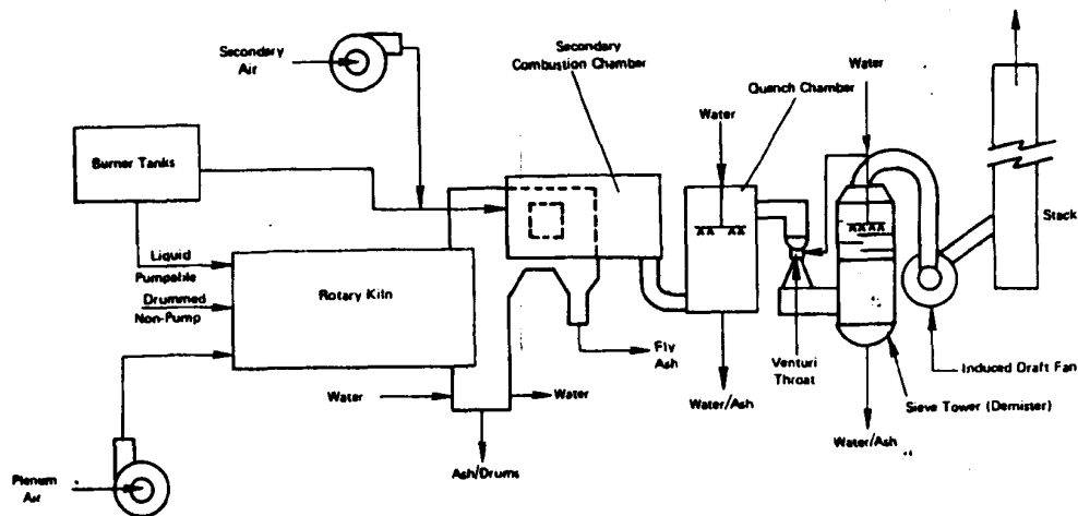
Figure 5-6. Schematic of Rotary Kiln Facility (Courtesy of 3M Company)
