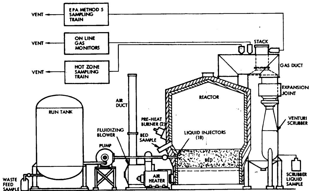
Figure 5-4. Systech Fluidized Bed Facility Schematic
