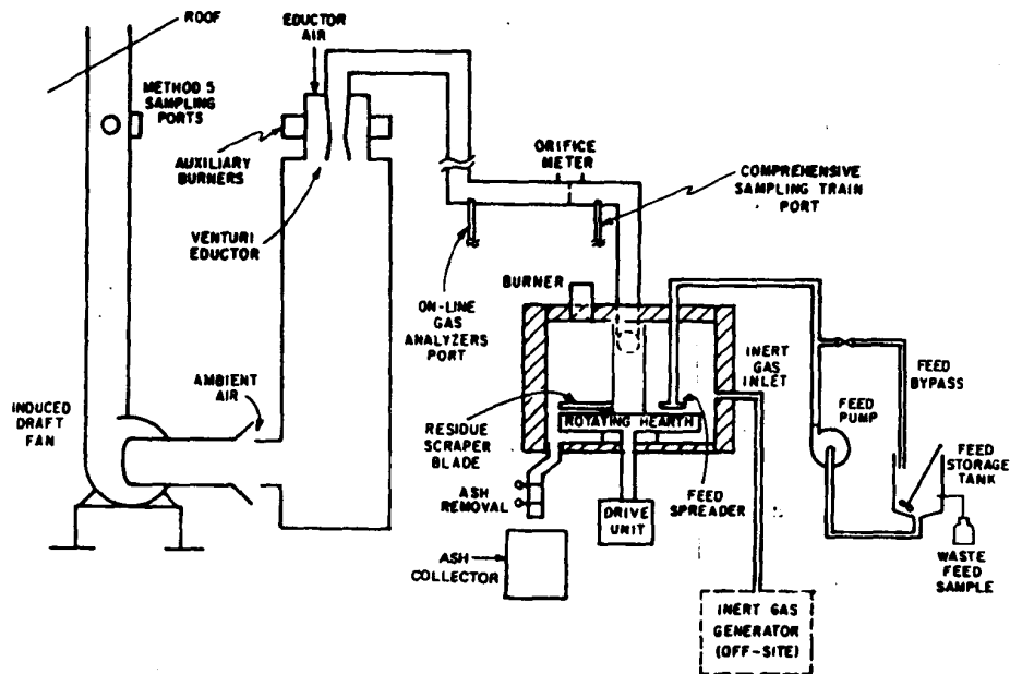
Figure 5-2. Schematic of Test Pyrolyzer/Incineration System
