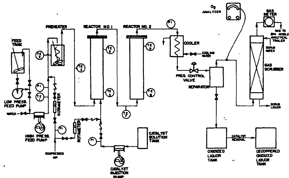
Figure 5-5. Flow Diagram of Mobile Industrial Pilot Plant Wet Oxidation
