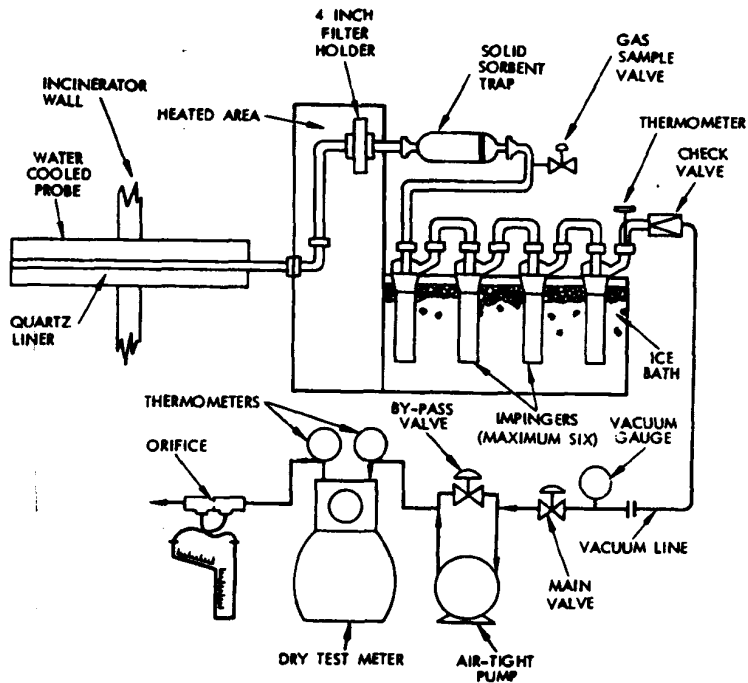
Figure 3-1. Combustion Zone Sampling Train Schematic
