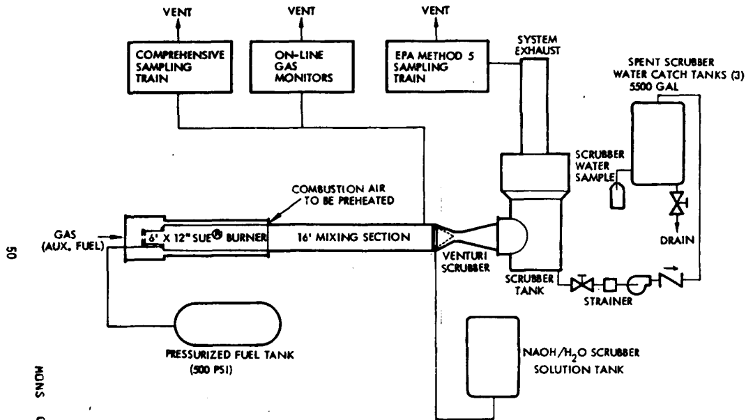
Figure 5-1. TMC Test Facility
