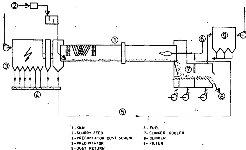
Figure 5-3. St. Lawrence Wet Process Cement Kiln Schematic (Courtesy of St. Lawrence Cement Co.)
