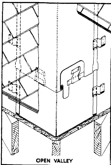
Drawing of correct installation of open valley flashing and two views showing one sheet being installed with supporting cleats and the finished valleys after re-ashing
