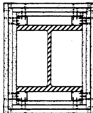
ILLUSTRATION—THREE-HOUR fire rated steel column assembly with \frac{1}{2} " Firestop. X509 (UL 18).
