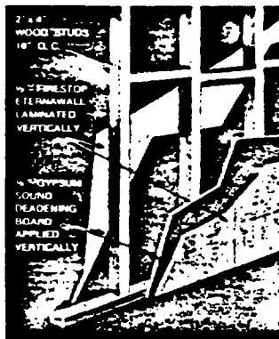
U.L. Design No. 30 Fire Rating—1 Hour Combustible STC-45
