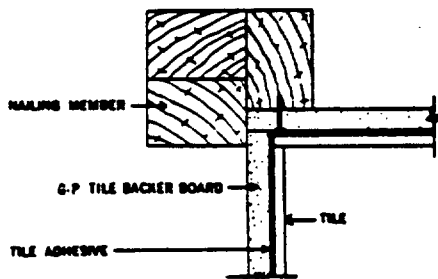
CORNER DETAIL
