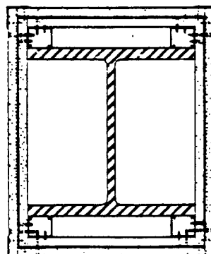
ILLUSTRATION—TWO HOUR fire rated steel column assembly with \frac{3}{8} " Firestop. X517 (UL 8).
