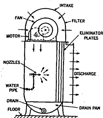
FIG. 20. HUMIDIFYING UNIT FOR WARM AIR FURNACE
