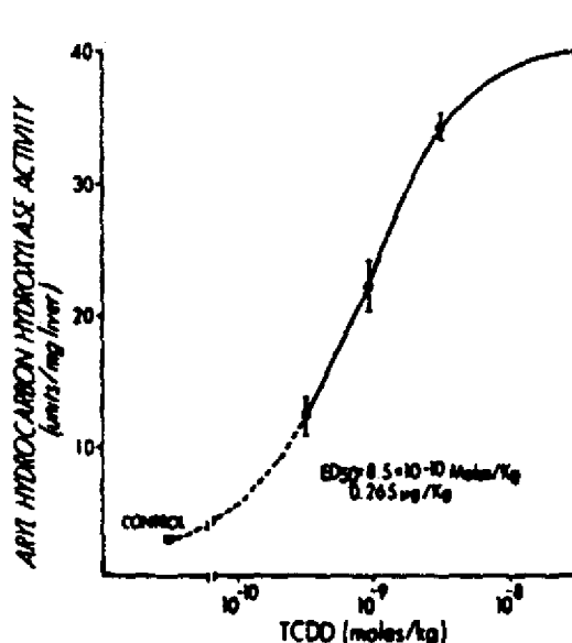
FIGURE 5. Logarithmic dose-response curve for the induction of aryl hydrocarbon hydroxylase in rat liver. Male Sprague-Dawley rats weighing about 80 g were injected intraperitoneally with TCDD dissolved in p -dioxane or p -dioxane alone ( 0.8 \text{ ml/kg} ), and hepatic aryl hydrocarbon hydroxylase activity was assayed 24 hr later. Each point is the mean \pm standard error of five animals.
