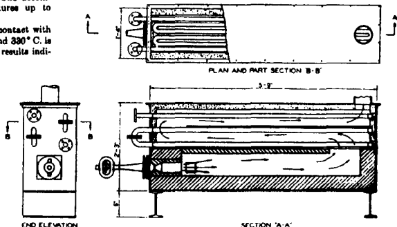
Figure 1. Heater
