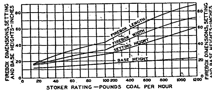
FIG. 11. SUGGESTED MINIMUM FIREBOX DIMENSIONS AND BASE HEIGHTS 2
