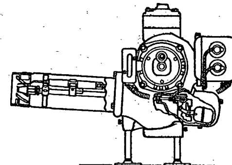
FIG. 12. LOW PRESSURE ATOMIZING OIL BURNER
