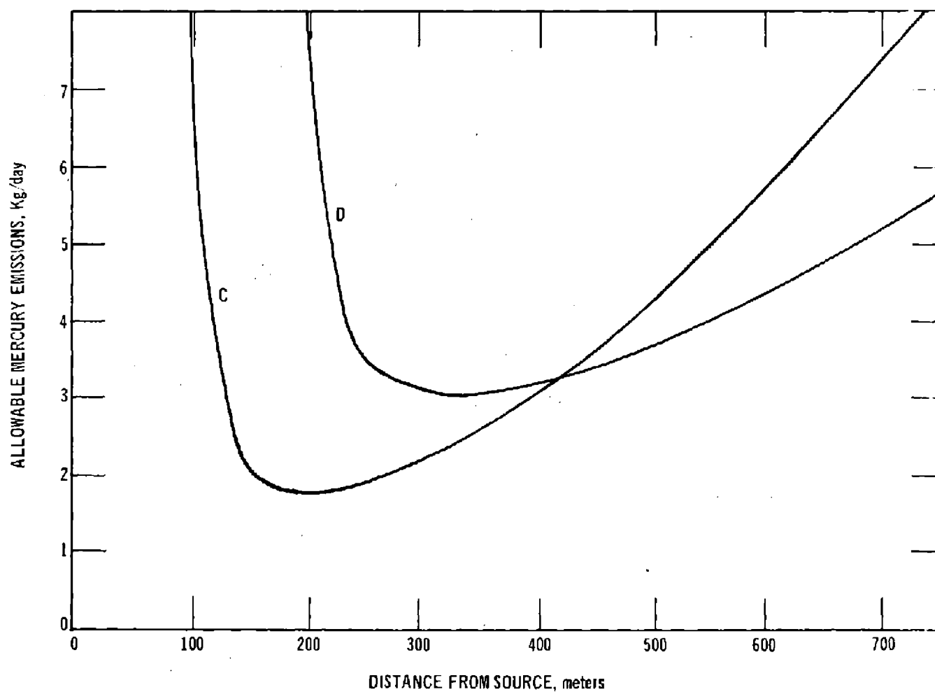
Figure C-1. Calculated maximum allowable mercury emissions from a sewage sludge incinerator under applicable Pasquill stability classes (C and D) and wind speed of 2 mps.
