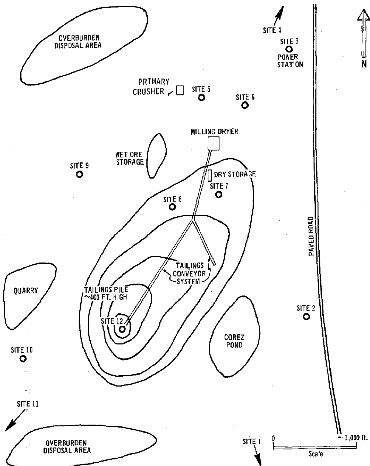
Figure 5-2. Sources of asbestos emissions in Hyde Park, Vermont.
