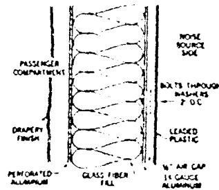
FIGURE 7. Section through the sound barrier used in HS Denison. It is basically similar to that used in the stationary turbine (Figure 4) except that lighter leaded vinyl sheet is employed and it is point-suspended for maximum limpness.
