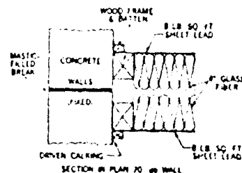
FIGURE 11. Section through the 70-db wall.
