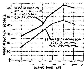
FIGURE 10. Acoustical performance of the original wall and the wall after sheet lead had been added clearly shows the improvement. (Original wall performance shown is estimated and probably quite conservative.) The curve for the leaded wall is not corrected for "flanking" or passage of sound around the wall.
