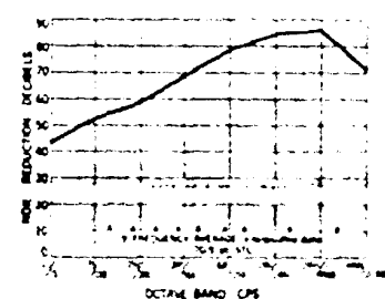
FIGURE 12. Actual performance of the 70-db wall as tested.
