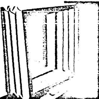
FIGURE 5. The flexible bellows (30 inches square) is used to connect the intake duct to the air intake of the turbine. It provides a reasonable transmission loss for noise without introducing a rigid structural tie between turbine and ducting.
