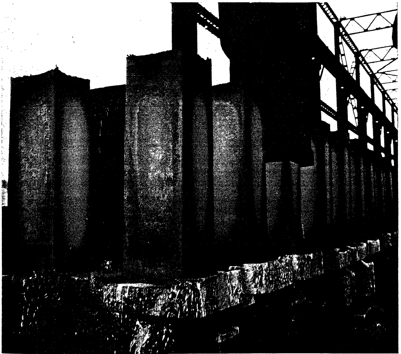
Removing molds (stripping) from hot Open Hearth ingots at the Lowellville, Ohio, Works of the Sharon Steel Corporation.
