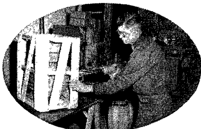
The door-like fourth side is folded shut and the wires are twisted closed with an electric toggle twister.
