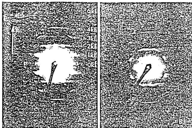
FIG. 2. Selected area electron diffraction patterns obtained on fibers of chrysotile obtained during air sampling at brake repair shops. In A, the reciprocal a^* axis is marked as are the layer lines in the (OKI) series. Indexing of upper right quadrant yielded 16 reflections corresponding to single crystal X-ray diffraction analysis of Whittaker and Zussman, 1936. Pattern in (B) displays "smearing" of reflections in a "clockwise" manner suggesting interplanar rotation.
