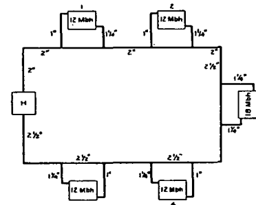
FIG. 7. A ONE-PIPE GRAVITY CIRCULATION SYSTEM
