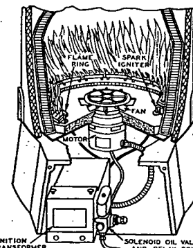
FIG. 15. WALL FLAME VERTICAL ROTARY BURNER
