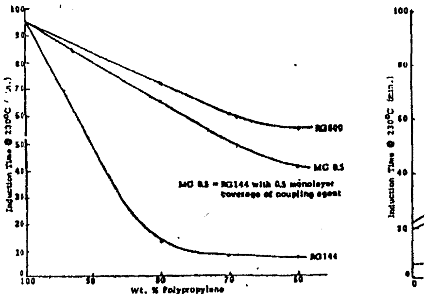
FIGURE 1 COUPLING AGENT EFFECTS ON THERMAL STABILITY OF CHRYSOITILE/POLYPROPYLENE BLENDS
