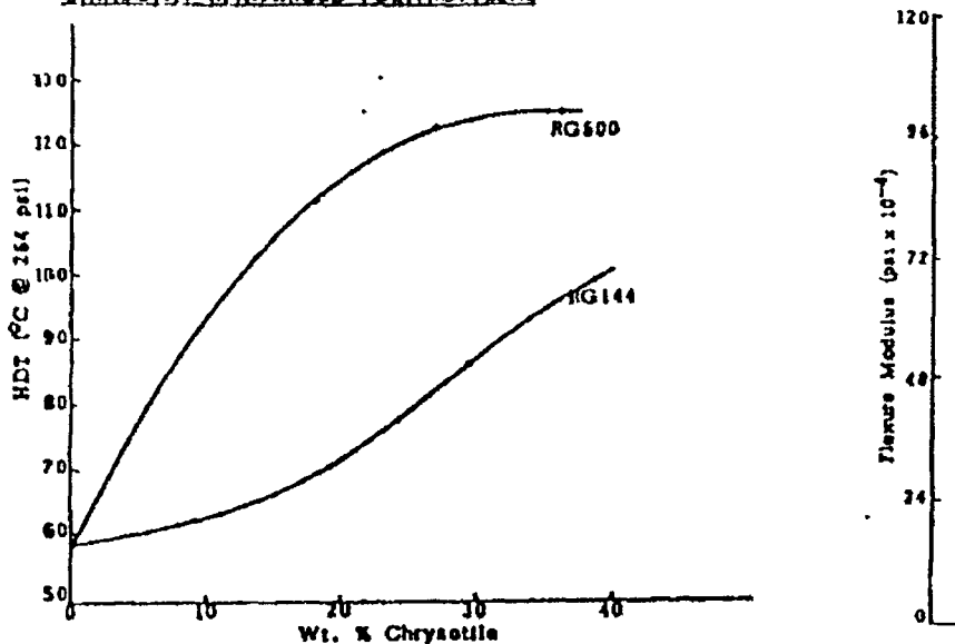
FIGURE 1 COUPLING AGENT EFFECTS ON THERMAL STABILITY OF CHRYSOITILE/POLYPROPYLENE BLENDS
