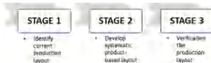
Fig. 11.1 Research methodology
