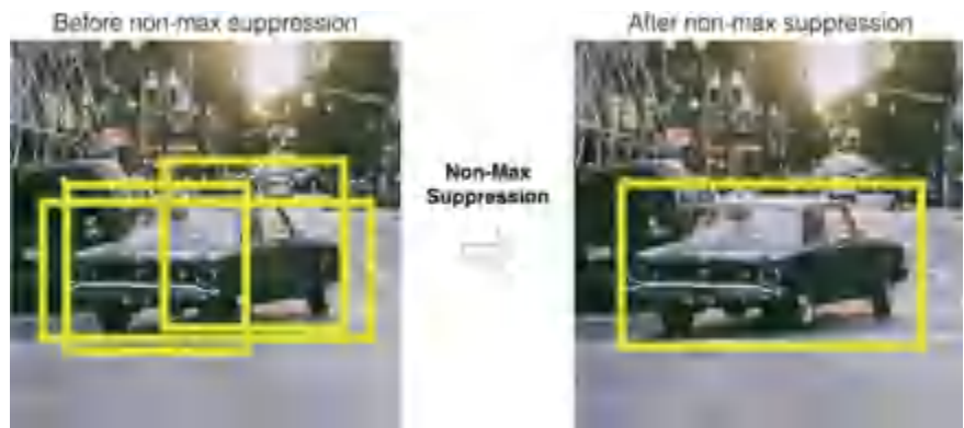
Fig. 4.5 Non-max suppression
