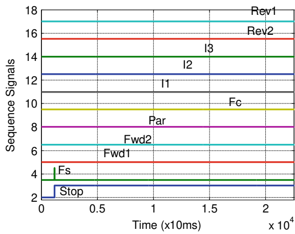
Fig. 15.9 Sequence signals with error
