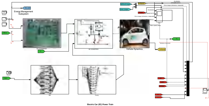
Fig. 16.5 MATLAB/Simulink model
