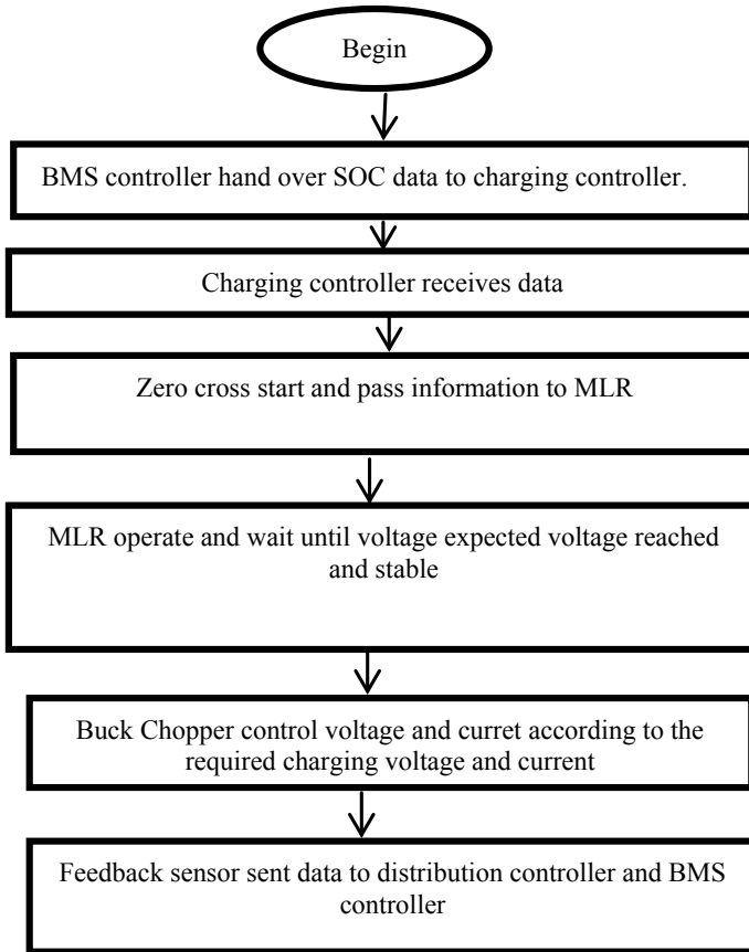
Fig. 19.4 Flow chart of BMS controller operation
