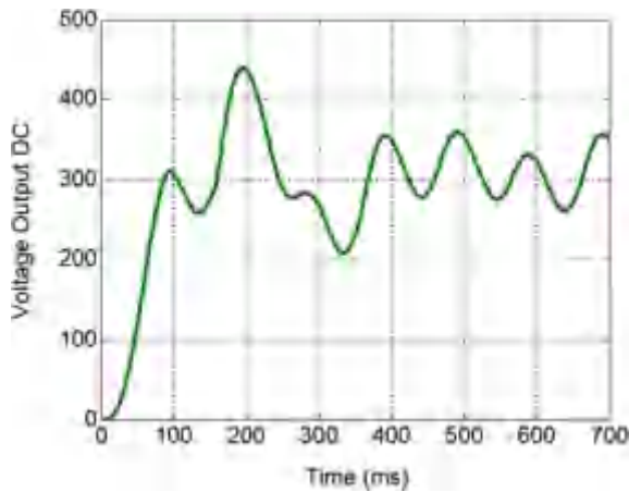
Fig. 18.9 Output voltage of MLR
