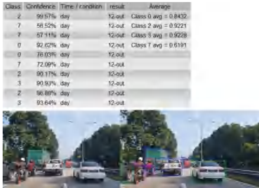
Fig. 4.9 Multiple class vehicle detection
