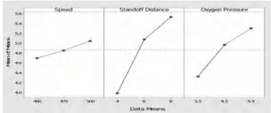
Fig. 21.1 Main effects plot for means of MRR
