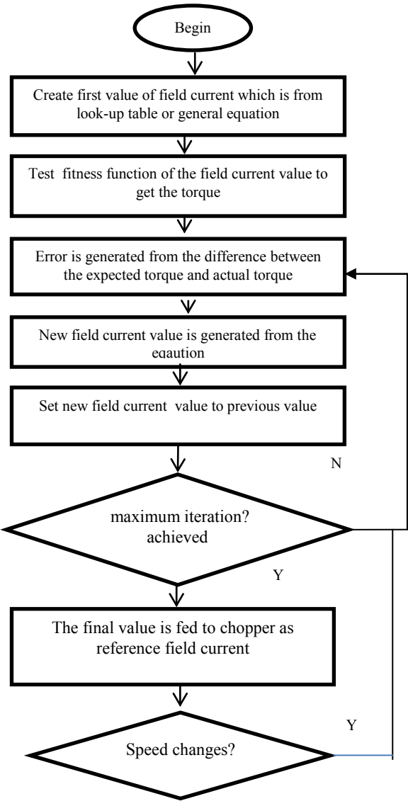
Fig. 16.3 Field weakening
