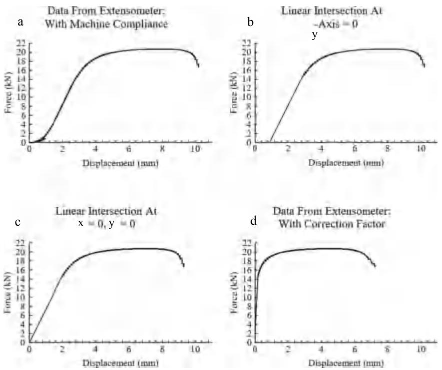
Fig. 10.3 The four stages in removing machine compliance from the force-displacement response of the tensile test. Figure a is the force-displacement response with the effect of machine compliance. Figure b is to correct the linear-elastic region of the curve. Figure c is to bring the starting position to zero. Figure d is the final curve for the specimen elongation with applied correction factor
