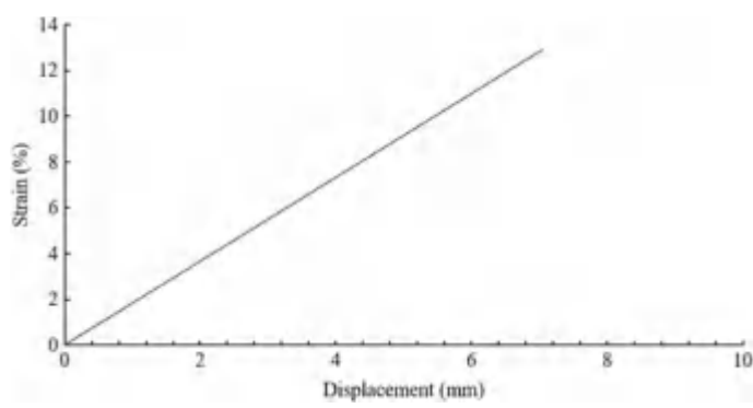
Fig. 10.6 Strain and displacement measurements obtained using optical 2D DIC virtual strain gauge
