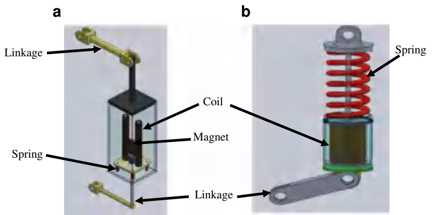
Fig. 26.2 a Design 1. b Design 2
