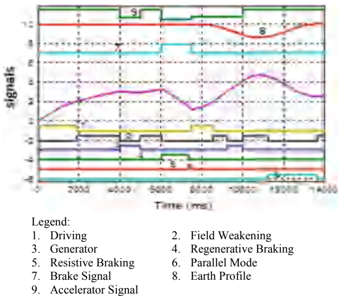
Fig. 14.4 FQDC operation results
