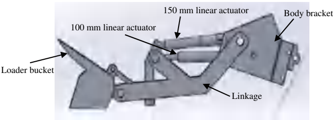
Fig. 30.8 Side view of loader bucket
