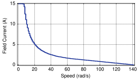
Fig. 16.8 Look-up table of field current versus speed
