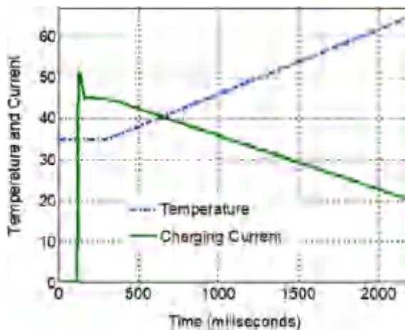
Fig. 18.13 Controlling charging current to control temperature
