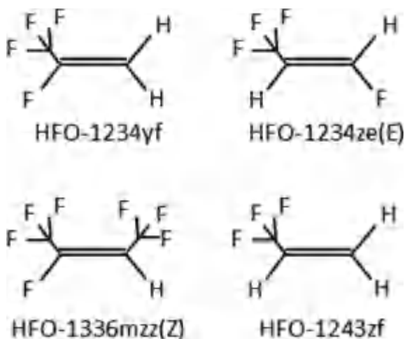
Fig. 27.6 Structural formula of some HFOs
