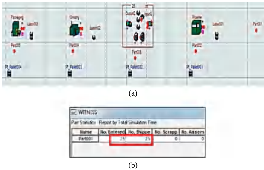
Fig. 13.4 a The simulation structure of the new layout, b the simulation of daily production for new layout for first proposal using I-Line
