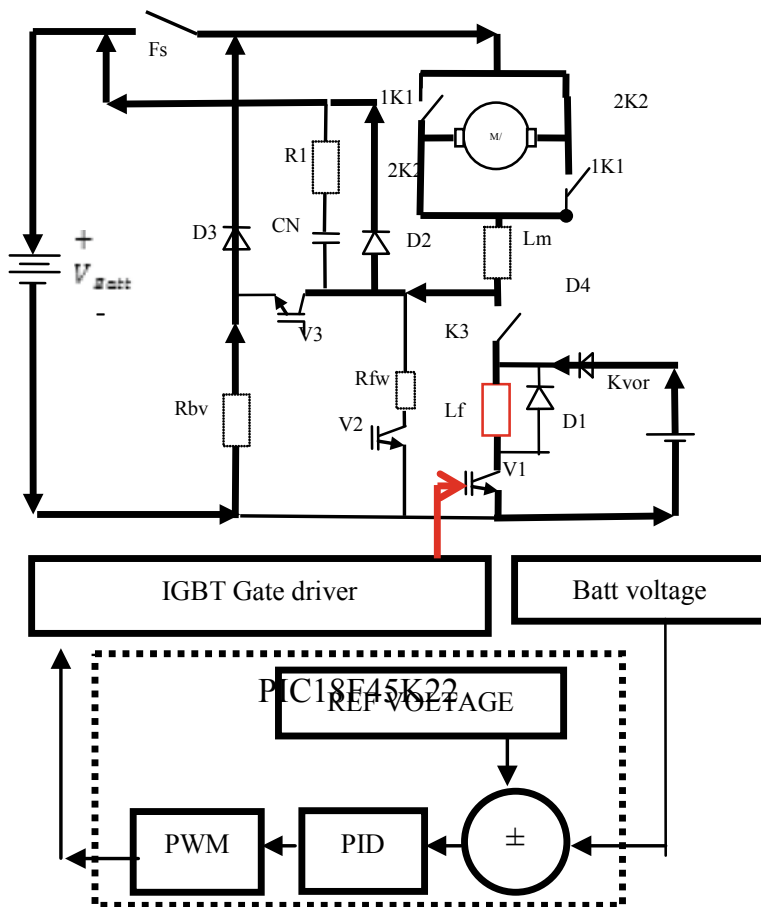
Fig. 15.1 New four quadrants DC chopper
