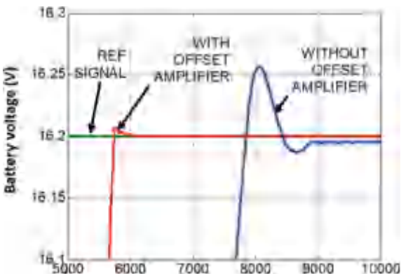
Fig. 18.12 Comparison of circuits with and without zooming effect
