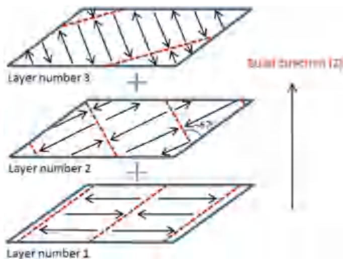
Fig. 9.9 Rotated strip pattern
