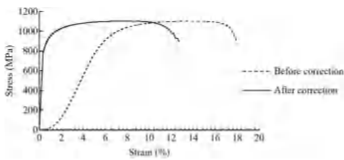
Fig. 10.5 Stress-strain curves comparison between before and after applying the correction factor
