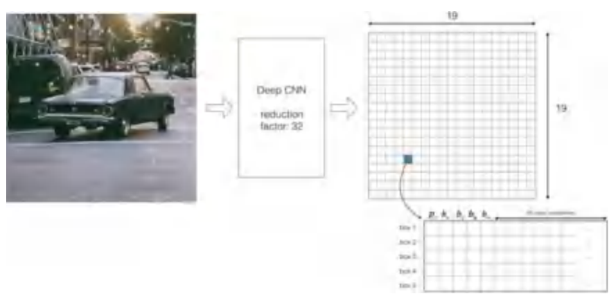
Fig. 4.4 Splitting the image into a cell
