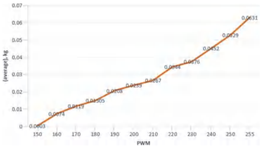
Fig. 3.9 Graph of the average weight exerted on the strain gauge load cell versus PWM
