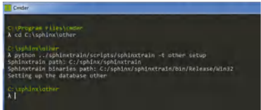
Fig. 6.5 Sphinxtrain setup
