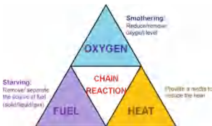
Fig. 27.1 Fire triangle
