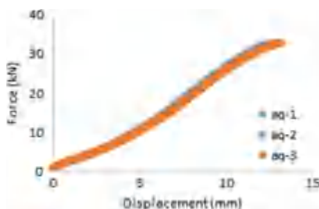
Fig. 24.4 Force-displacement response obtained from conducting punch test plotted according the tempering conditions
