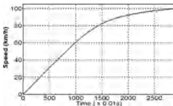
Fig. 17.8 Acceleration test
