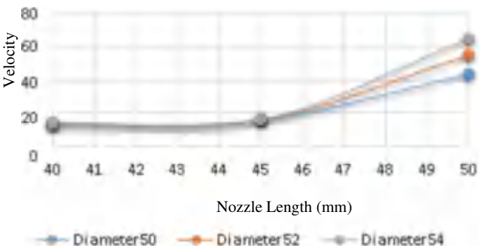
Fig. 28.10 Outlet 2 velocity curve
