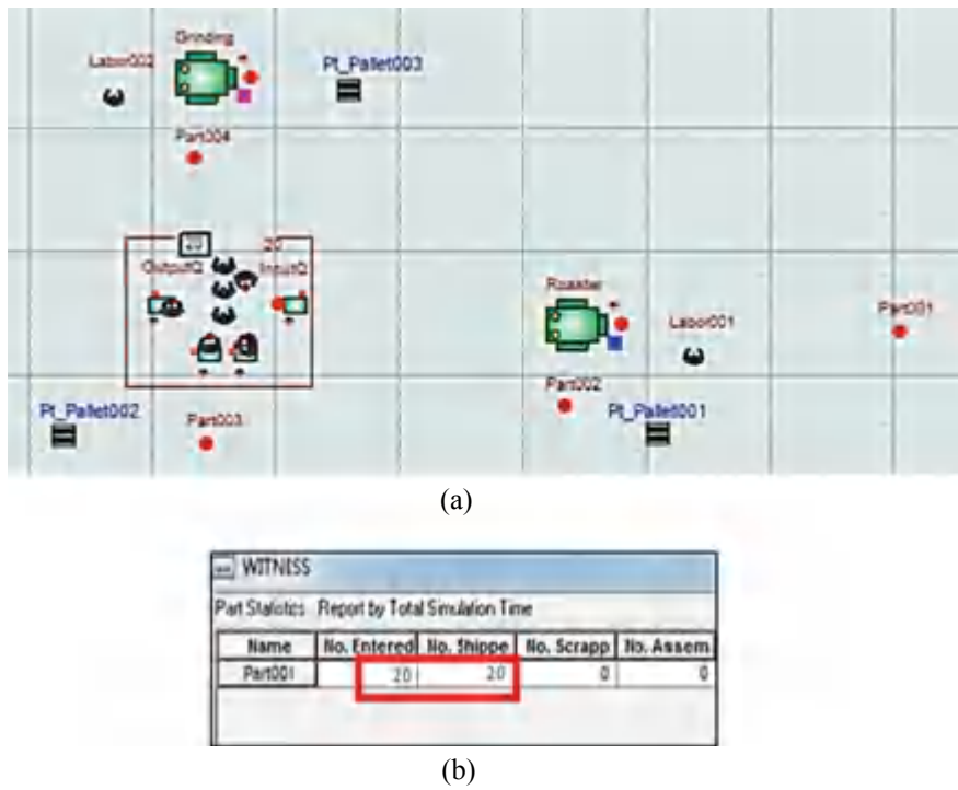
Fig. 13.5 a The simulation structure of the new layout, b the simulation of daily production for new layout for second proposal using L-Line
