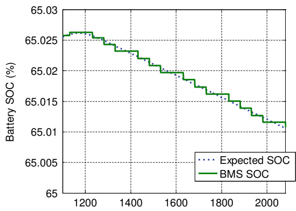
Fig. 19.11 SOC value when discharging
