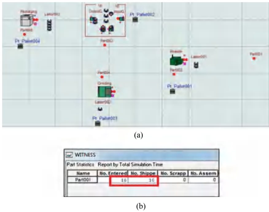
Fig. 13.3 a The simulation structure of the current layout, b the simulation of daily production for the current layout
