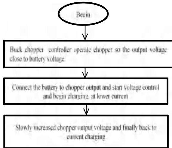
Fig. 18.5 Buck chopper controller control charging current operation
