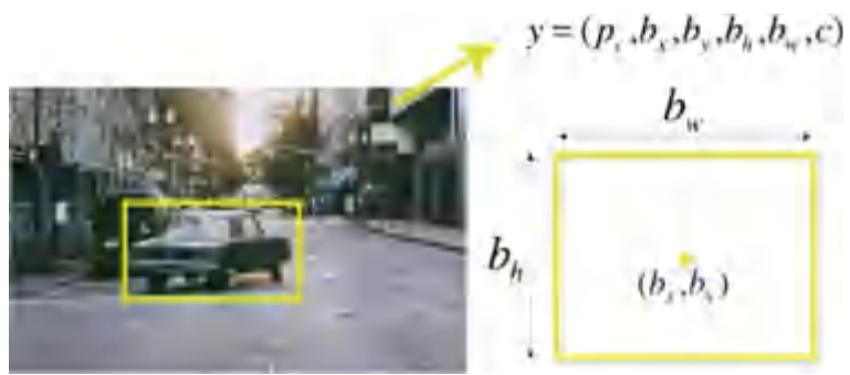
Fig. 4.3 The YOLO vehicle detection system
