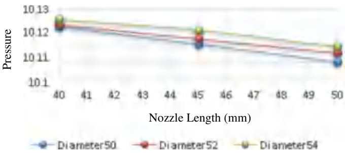
Fig. 28.9 Outlet 2 pressure curve
