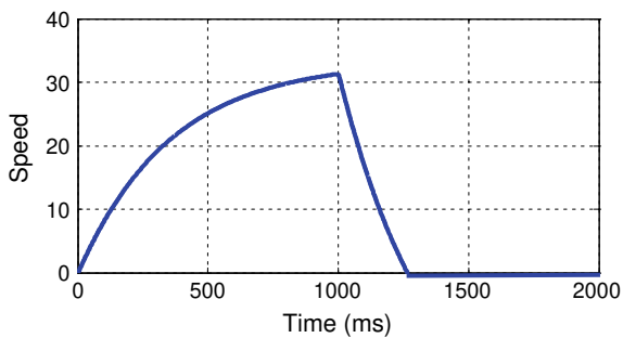
Fig. 20.4 speed pattern with braking action
