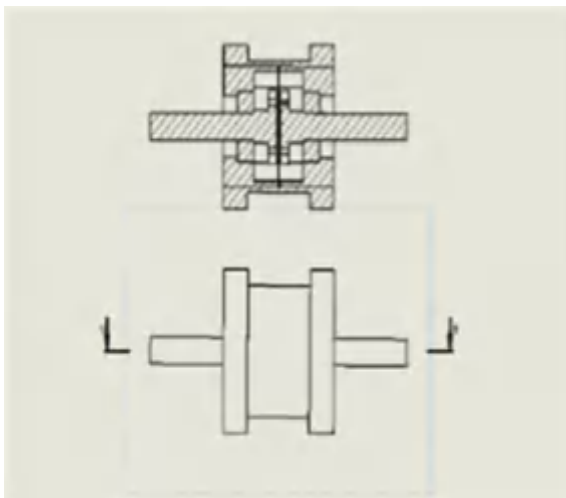
Fig. 3.5 Cross-section of the MRF transmission system
