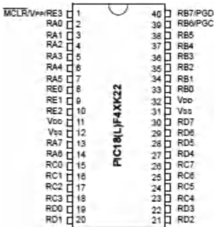
Fig. 19.2 PIC microcontroller
