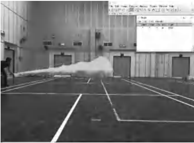
Fig. 28.6 Experimenting nozzle design with mode 2
