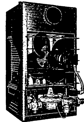
Cut-away view of heater, showing the cast iron heat exchanger in place.
