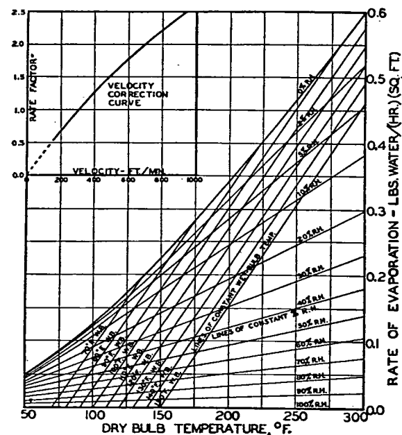
FIG. 8. RATE OF EVAPORATION CHART 2
