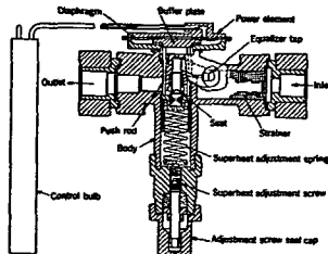
Fig. 15.... Typical Thermostatic Expansion Valve
