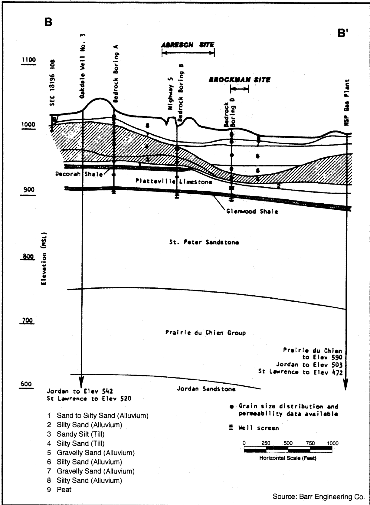
Figure 3 GEOLOGIC CROSS SECTION B-B' OAKDALE DISPOSAL SITE, MN
