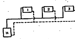
FIG. 5. A TWO-PIPE DIRECT RETURN SYSTEM
